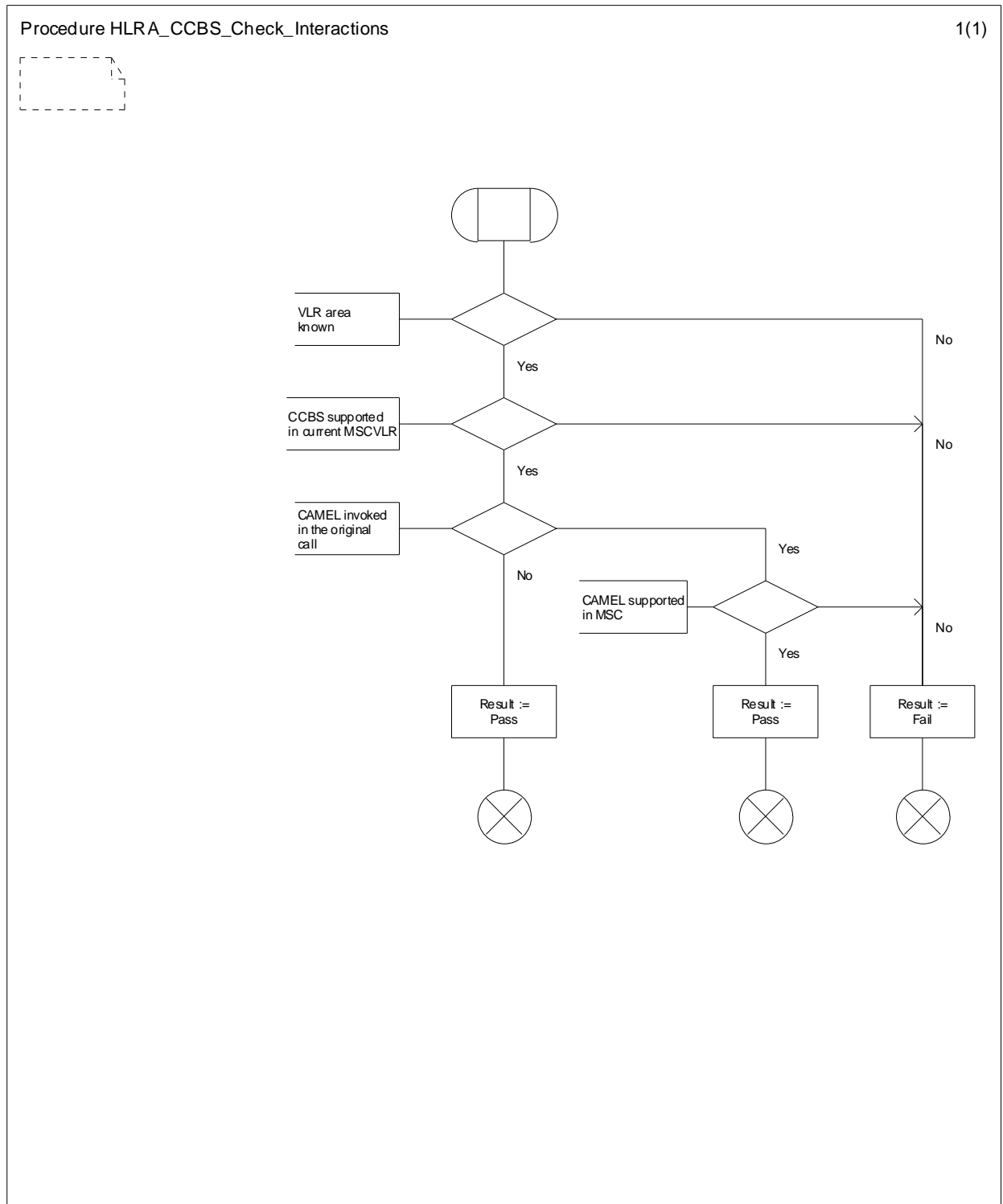
Figure 11.1.2.7: Procedure HLRA_CCBS_Check_Interactions
