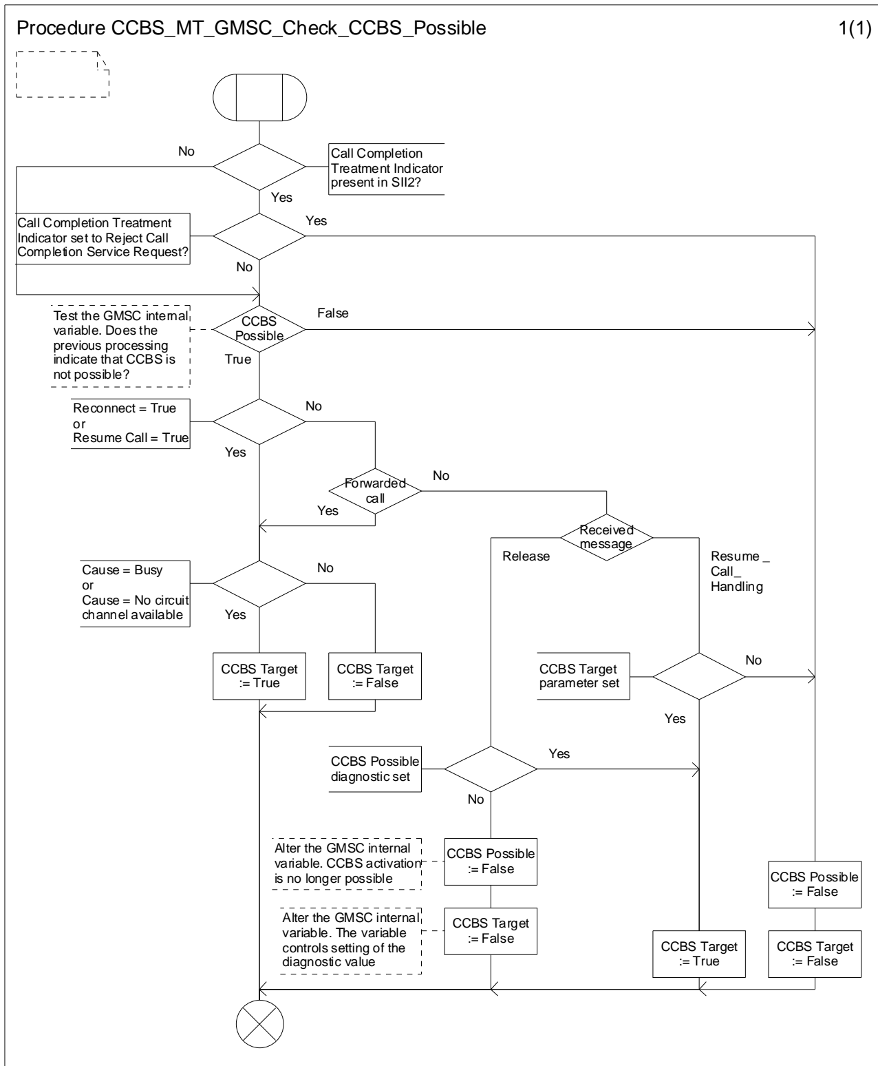
Figure 11.2.1.5: Procedure CCBS_MT_GMSC_Check_CCBS_Possible
