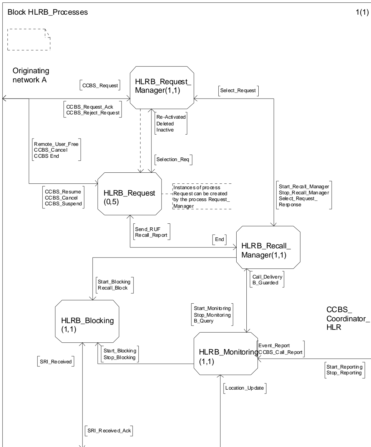
Figure 11.2.2.1: HLRB_Processes
