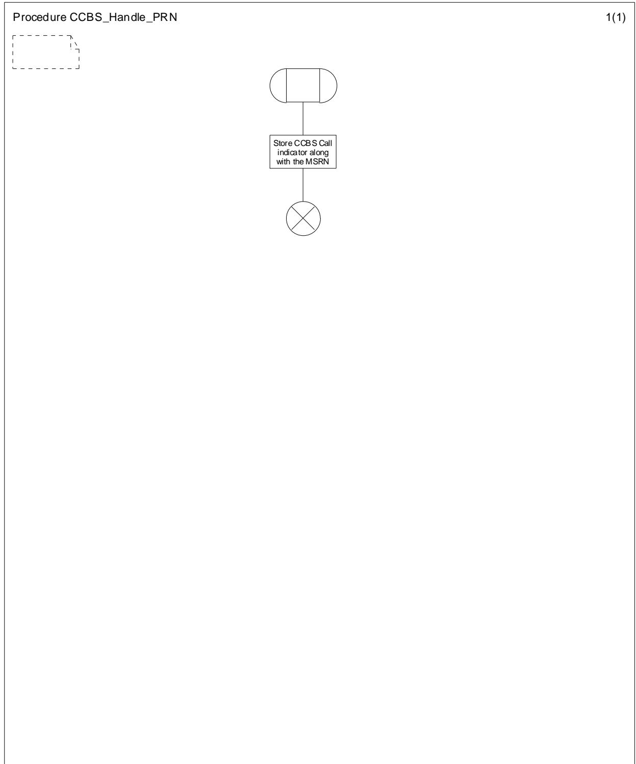
Figure 11.2.3.2: Procedure CCBS_Handle_PRN
