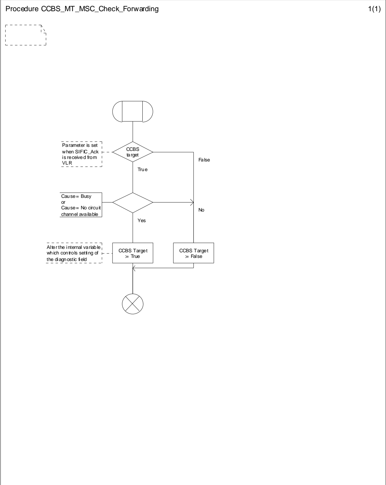
Figure 11.2.3.1: Procedure CCBS_MT_MSC_Check_Forwarding
