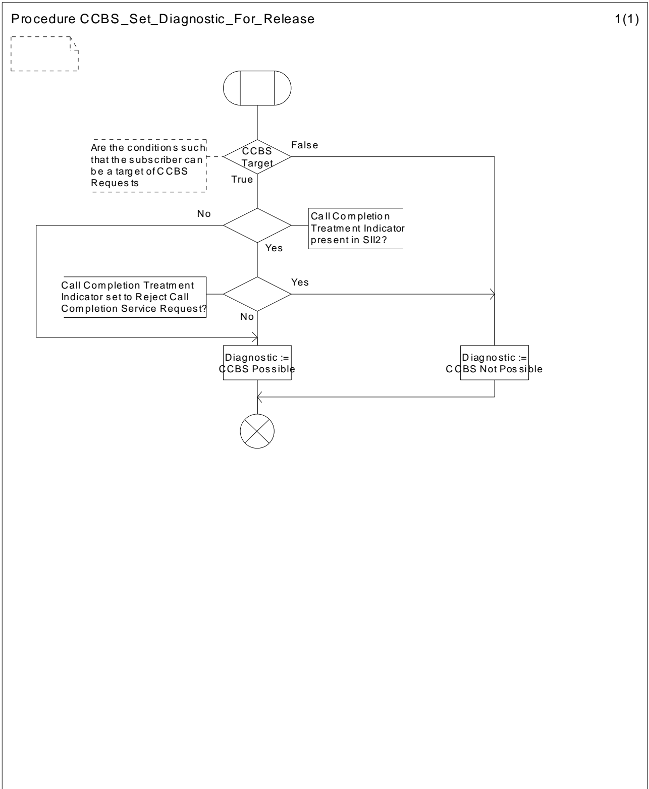
Figure 11.3.4: Procedure CCBS_Set_Diagnostic_For_Release
