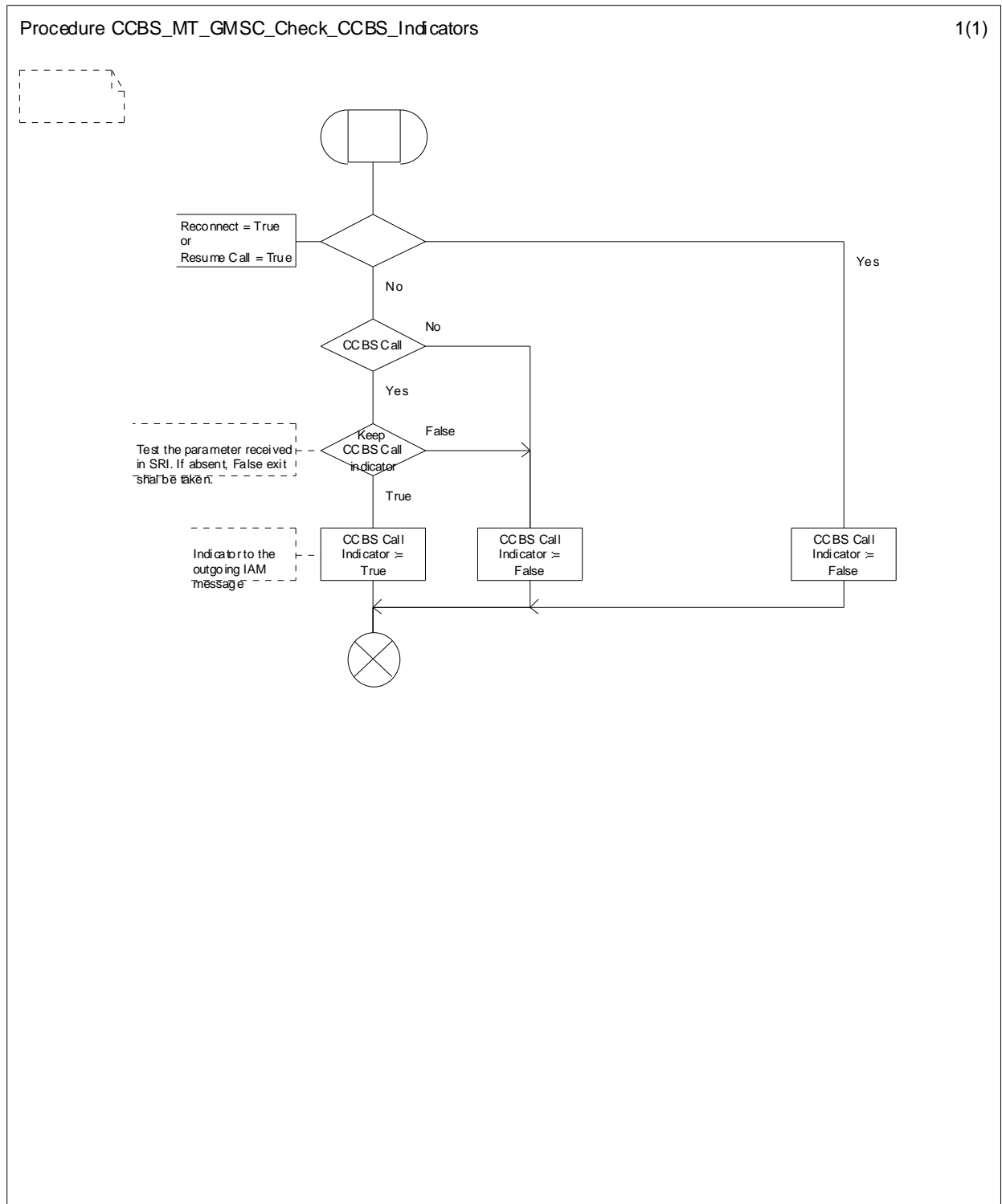
Figure 11.2.1.2: Procedure CCBS_MT_GMSC_Check_CCBS_Indicators
