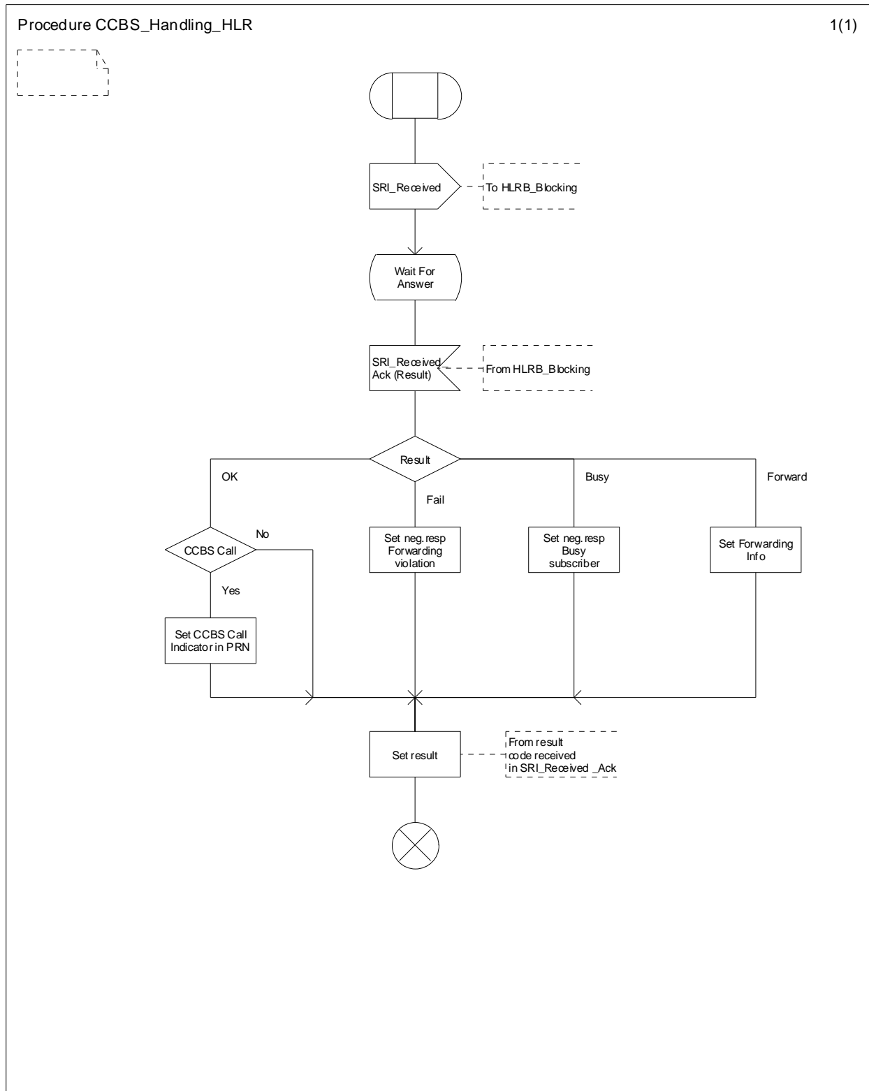
Figure 11.2.2.8: Procedure CCBS_Handling_HLR
