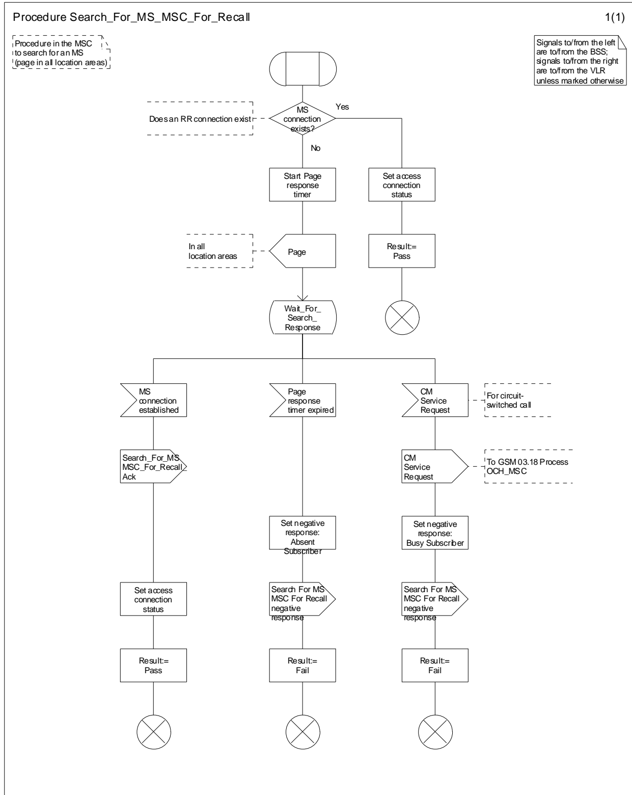
Figure 11.1.1.8: Procedure Search_For_MS_MSC_For_Recall
