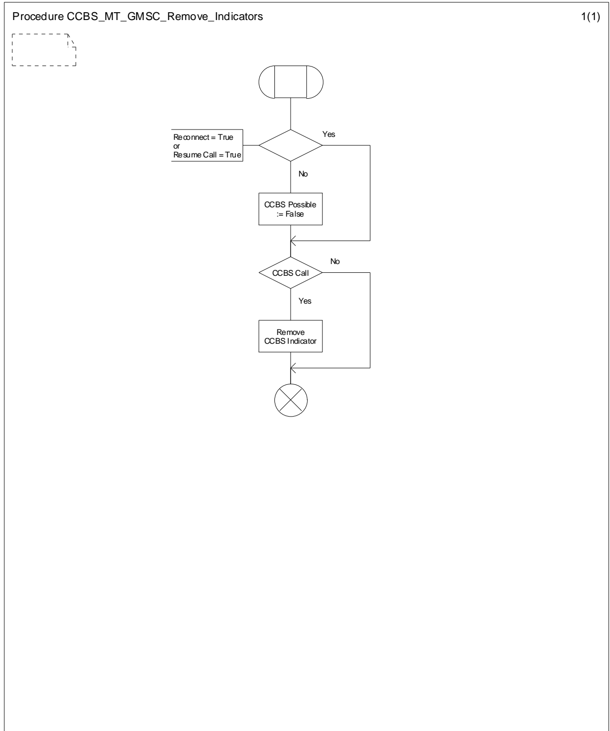
Figure 11.2.1.4: Procedure CCBS_MT_GMSC_Remove_Indicators
