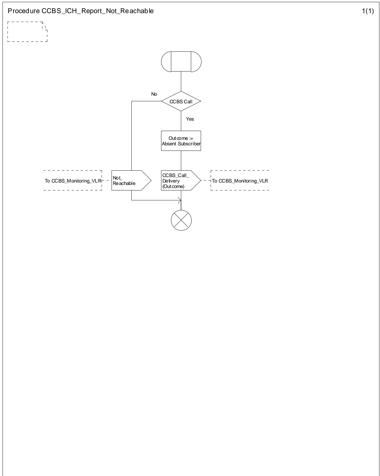
Figure 11.2.3.6: Procedure CCBS_ICH_Report_Not_Reachable
