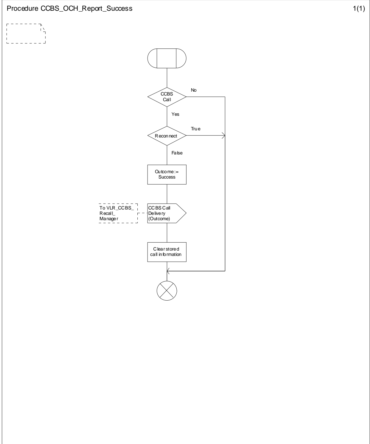
Figure 11.1.1.11: Procedure CCBS_OCH_Report_Success
