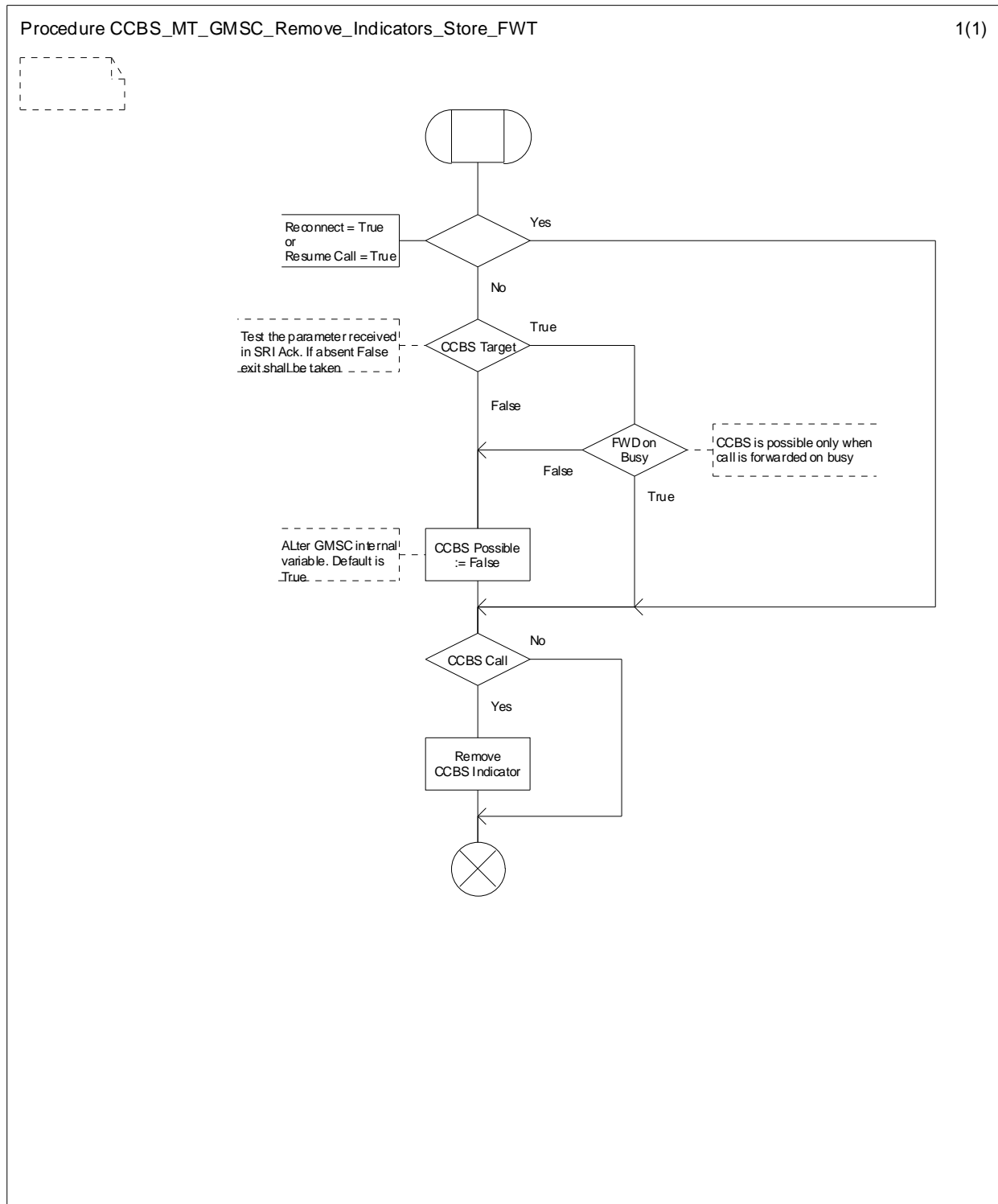
Figure 11.2.1.3: Procedure CCBS_MT_GMSC_Remove_Indicators_Store_FWT
