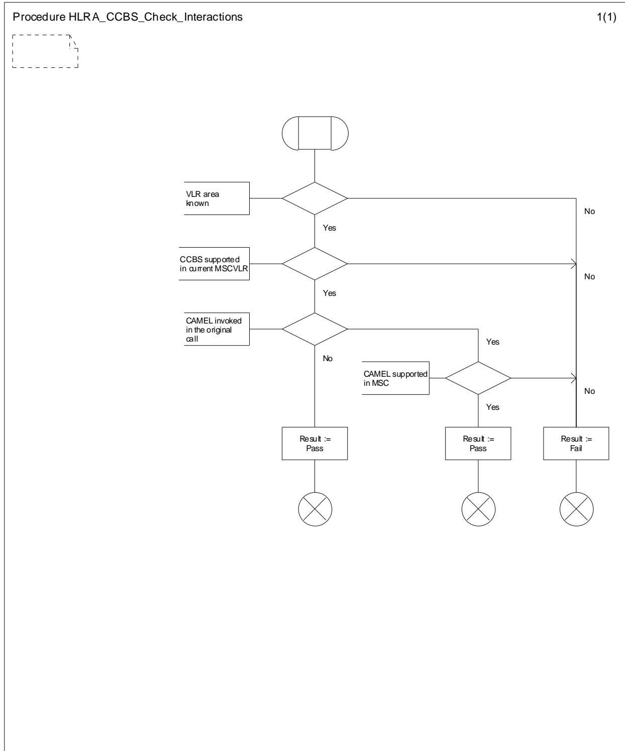
Figure 11.1.2.7: Procedure HLRA_CCBS_Check_Interactions
