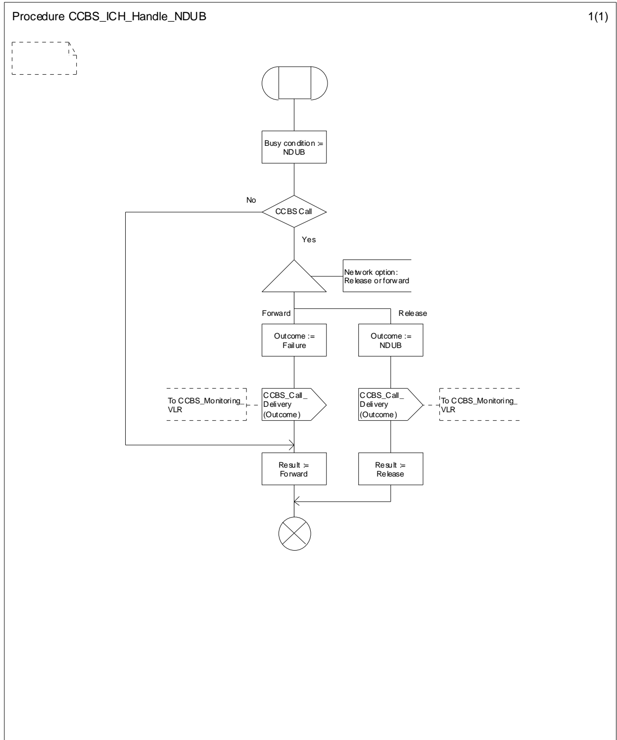
Figure 11.2.3.7: Procedure CCBS_ICH_Handle_NDUB
