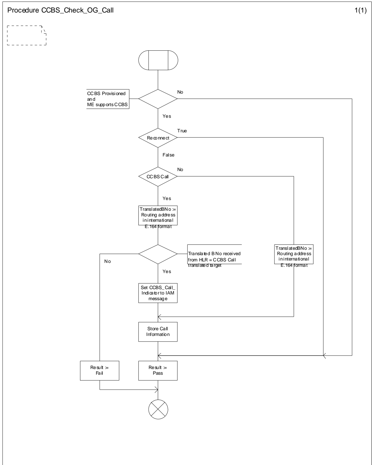
Figure 11.1.1.4: Procedure CCBS_Check_OG_Call
