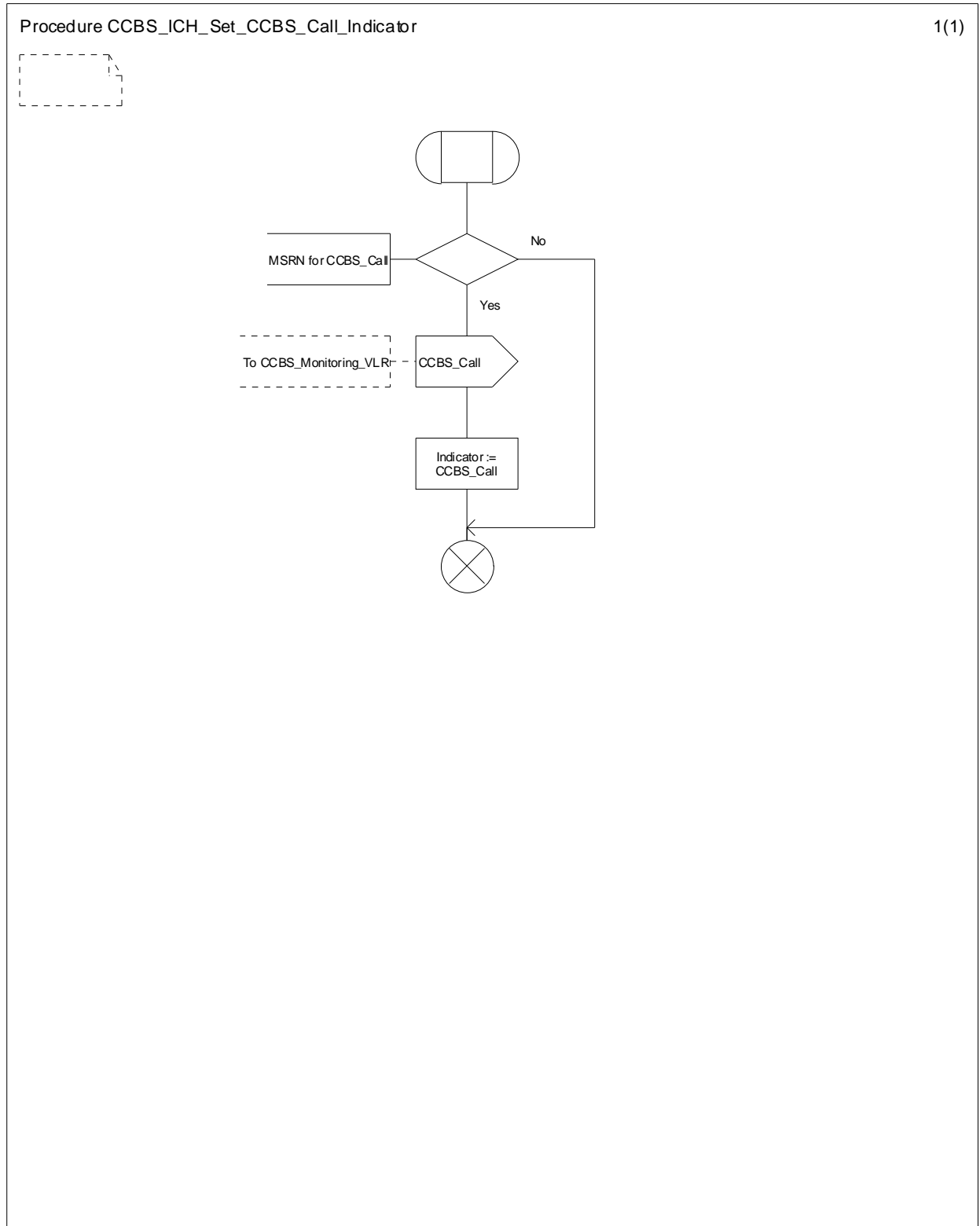
Figure 11.2.3.3: Procedure CCBS_ICH_Set_CCBS_Call_Indicator
