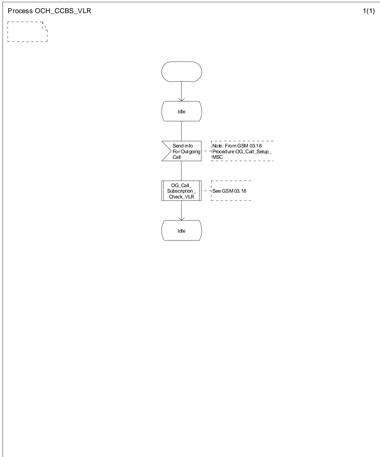
Figure 11.1.1.3: Process OCH_CCBS_VLR
