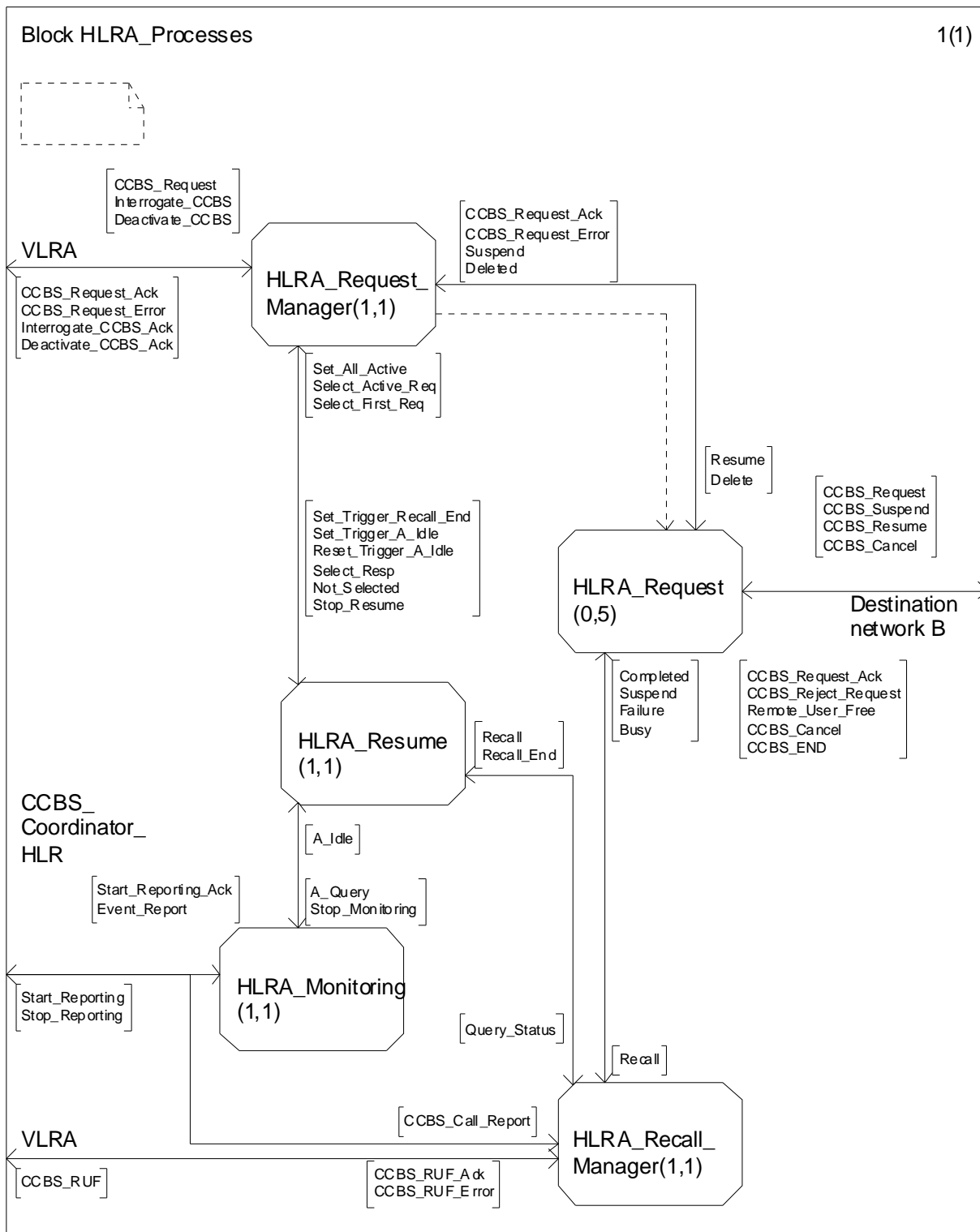
Figure 11.1.2.1: HLRA Processes
