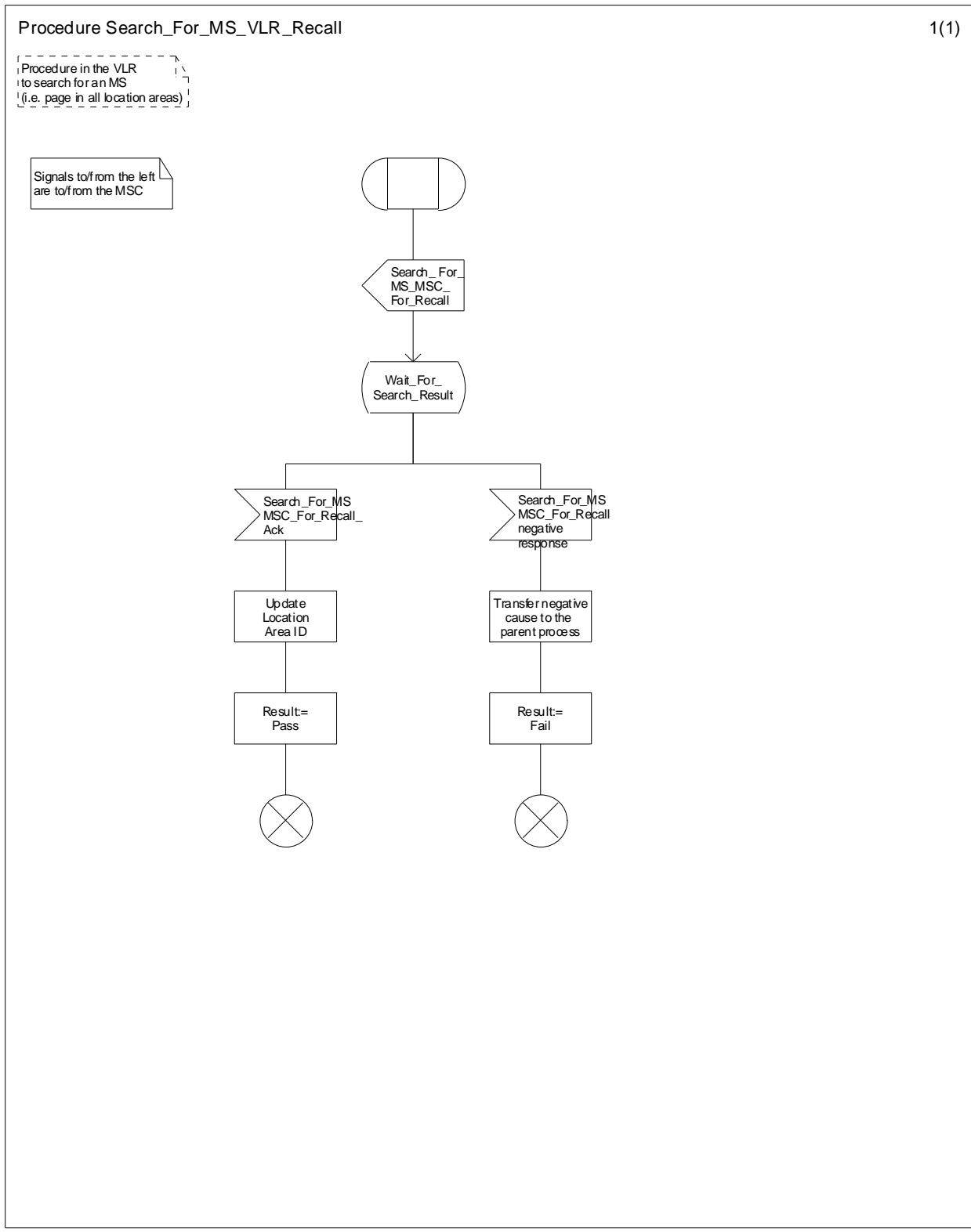
Figure 11.1.1.9: Procedure Search_For_MS_VLR_Recall
