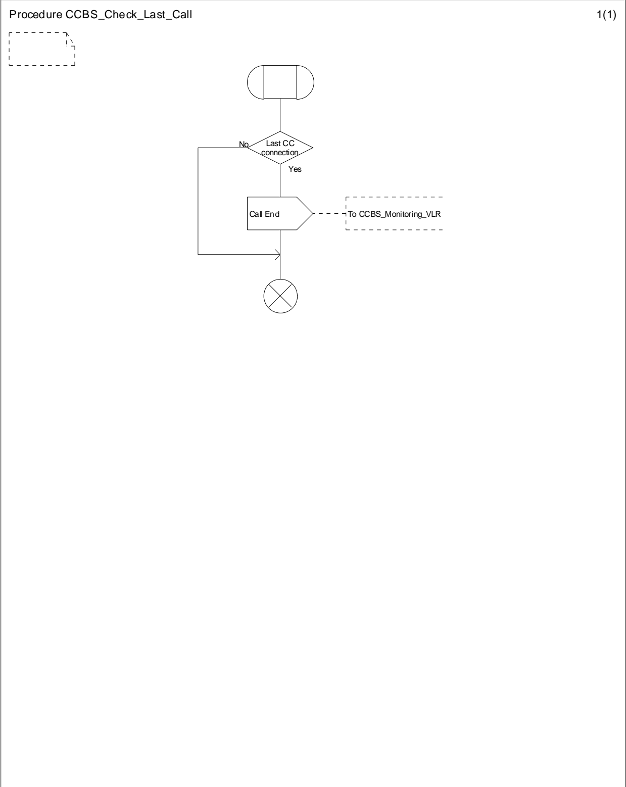
Figure 11.3.7: Procedure CCBS_Check_Last_Call
