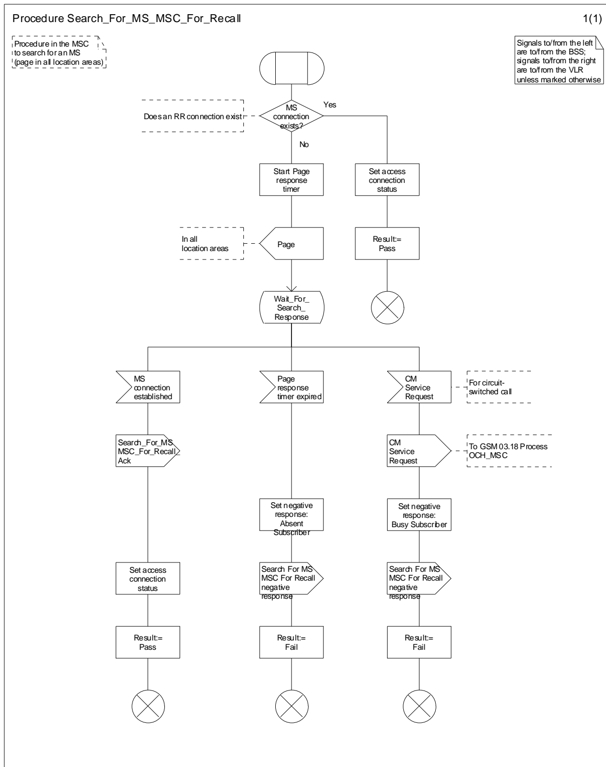
Figure 11.1.1.8: Procedure Search_For_MS_MSC_For_Recall
