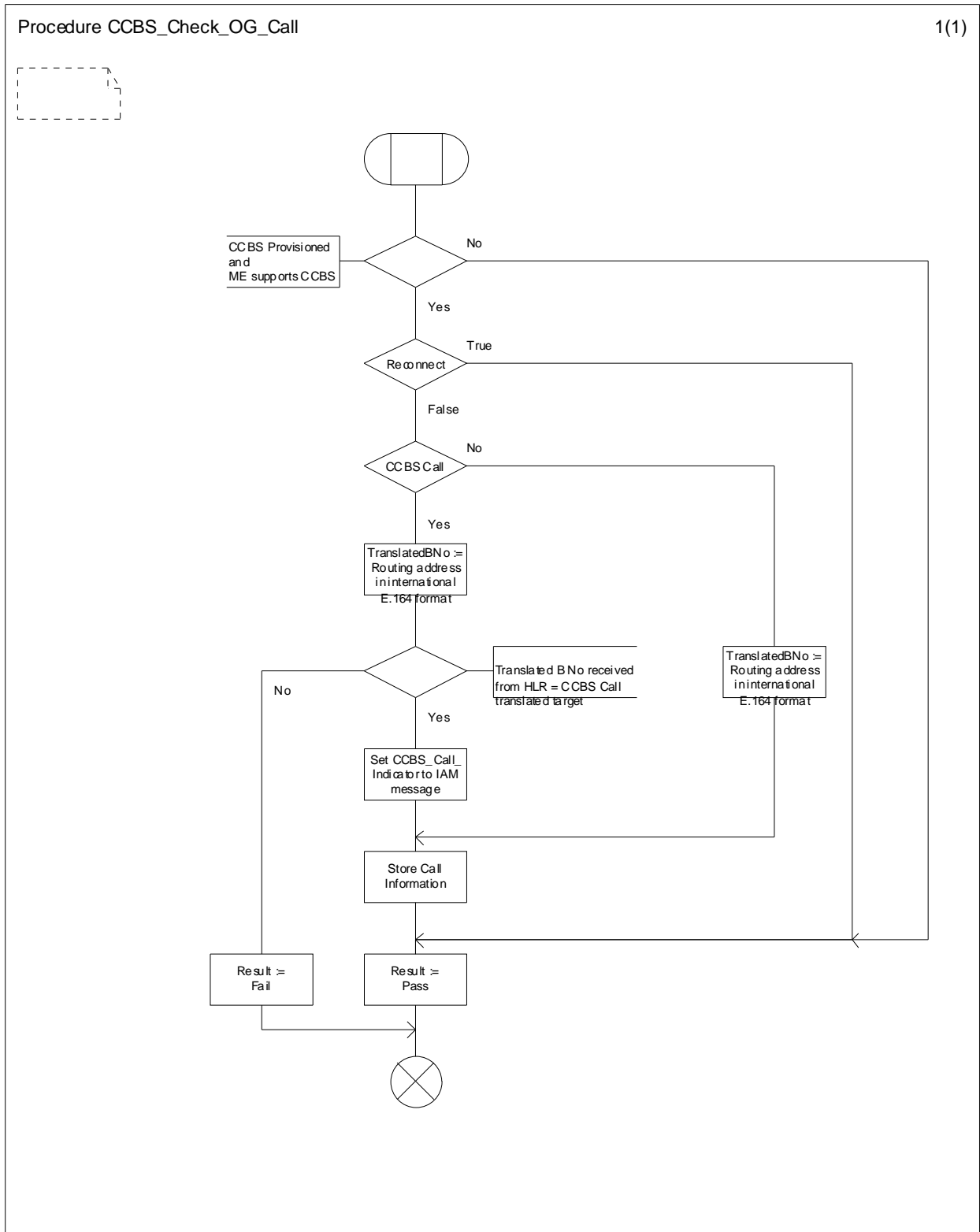
Figure 11.1.1.4: Procedure CCBS_Check_OG_Call
