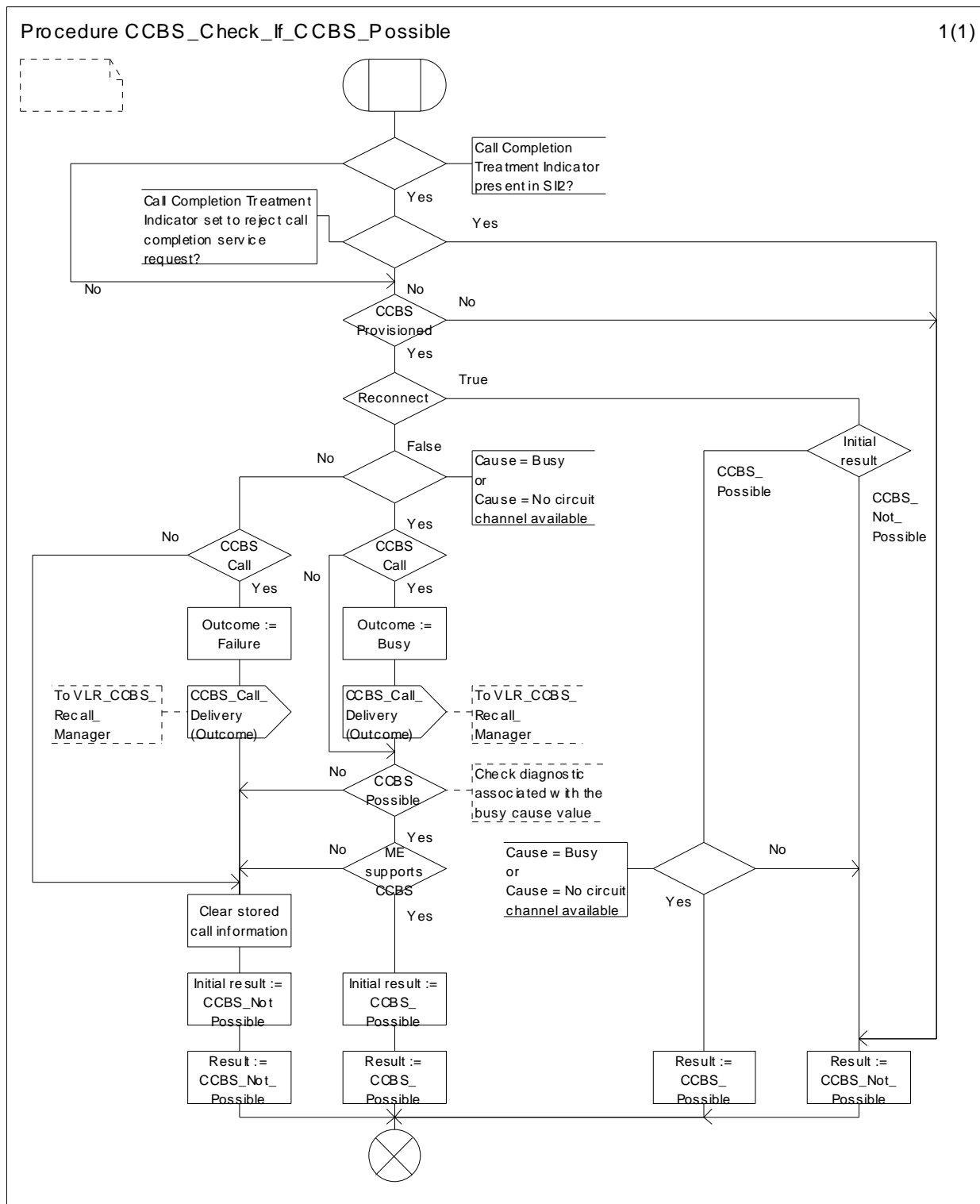
Figure 11.1.1.5: Procedure CCBS_Check_If_CCBS_Possible
