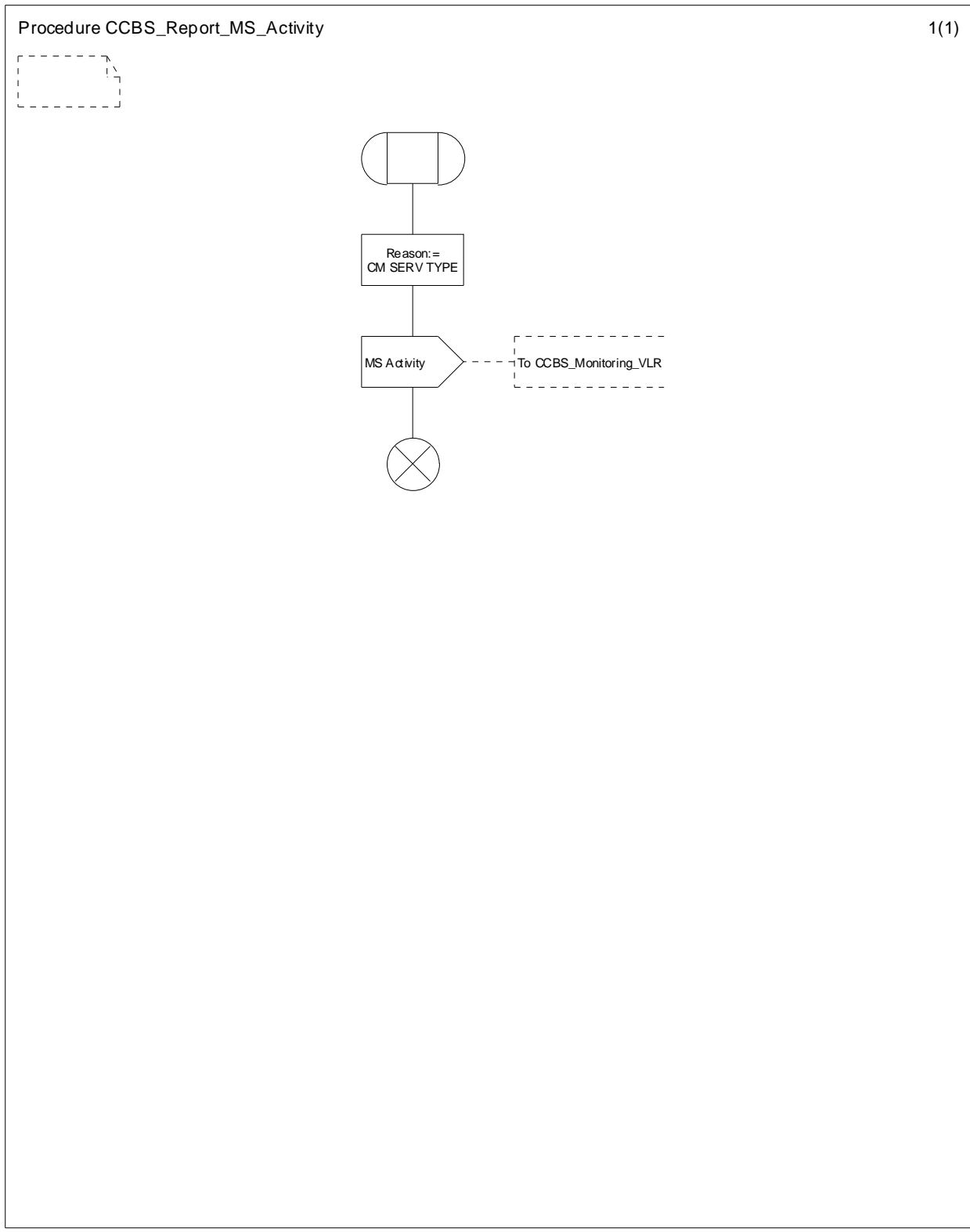
Figure 11.3.6: Procedure CCBS_Report_MS_Activity
