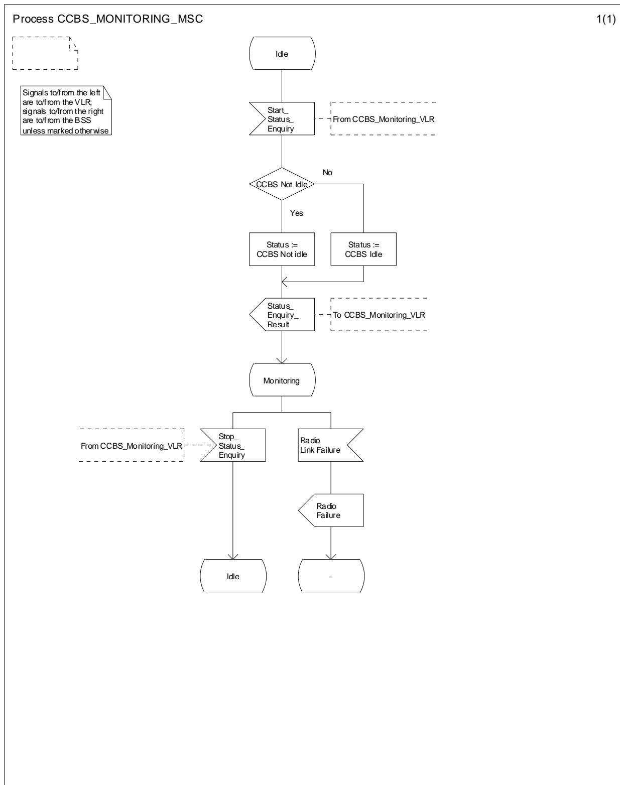
Figure 11.3.2: Process CCBS_Monitoring_MSC
