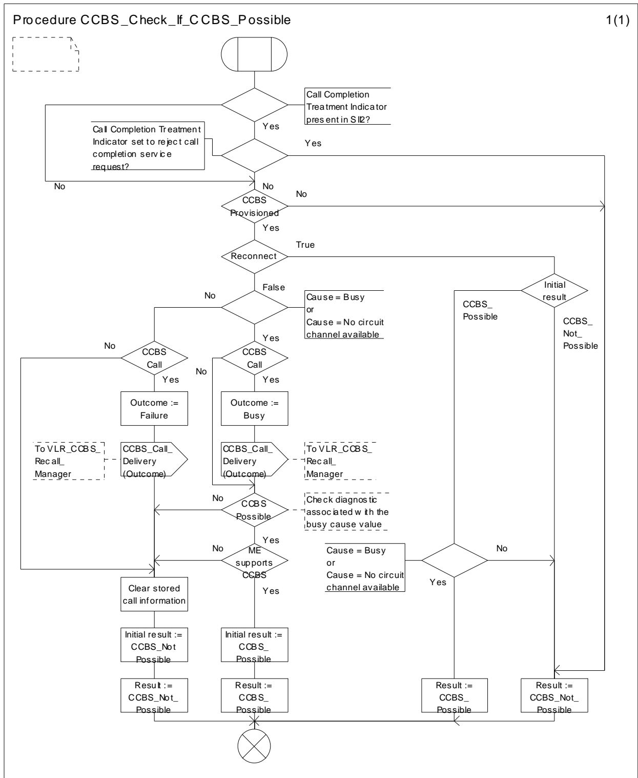
Figure 11.1.1.5: Procedure CCBS_Check_If_CCBS_Possible
