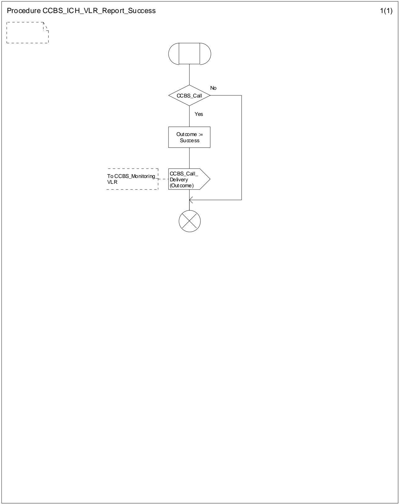
Figure 11.2.3.10: Procedure CCBS_ICH_VLR_Report_Success
