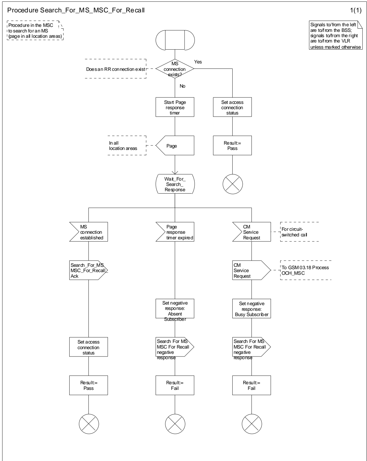
Figure 11.1.1.8: Procedure Search_For_MS_MSC_For_Recall
