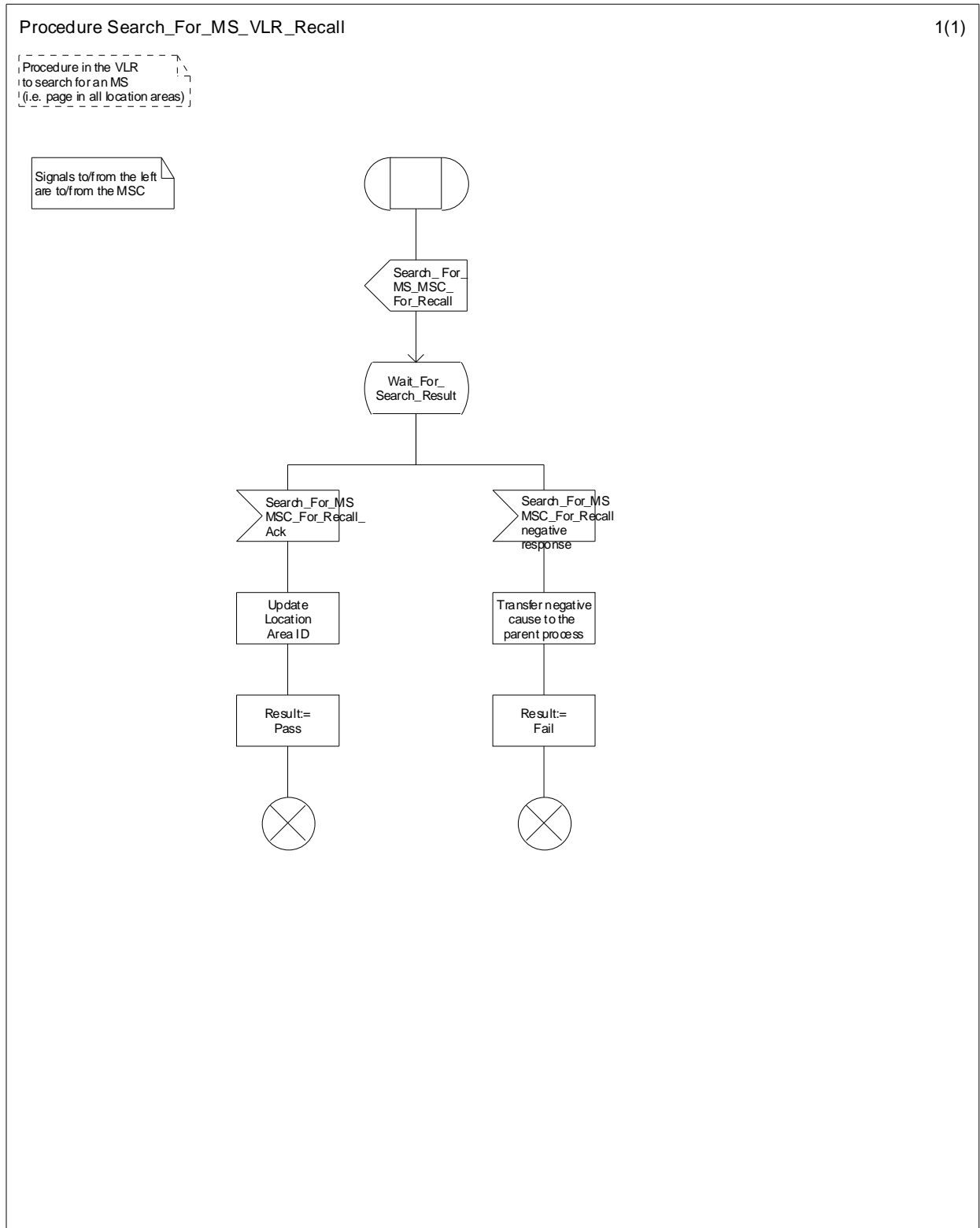
Figure 11.1.1.9: Procedure Search_For_MS_VLR_Recall
