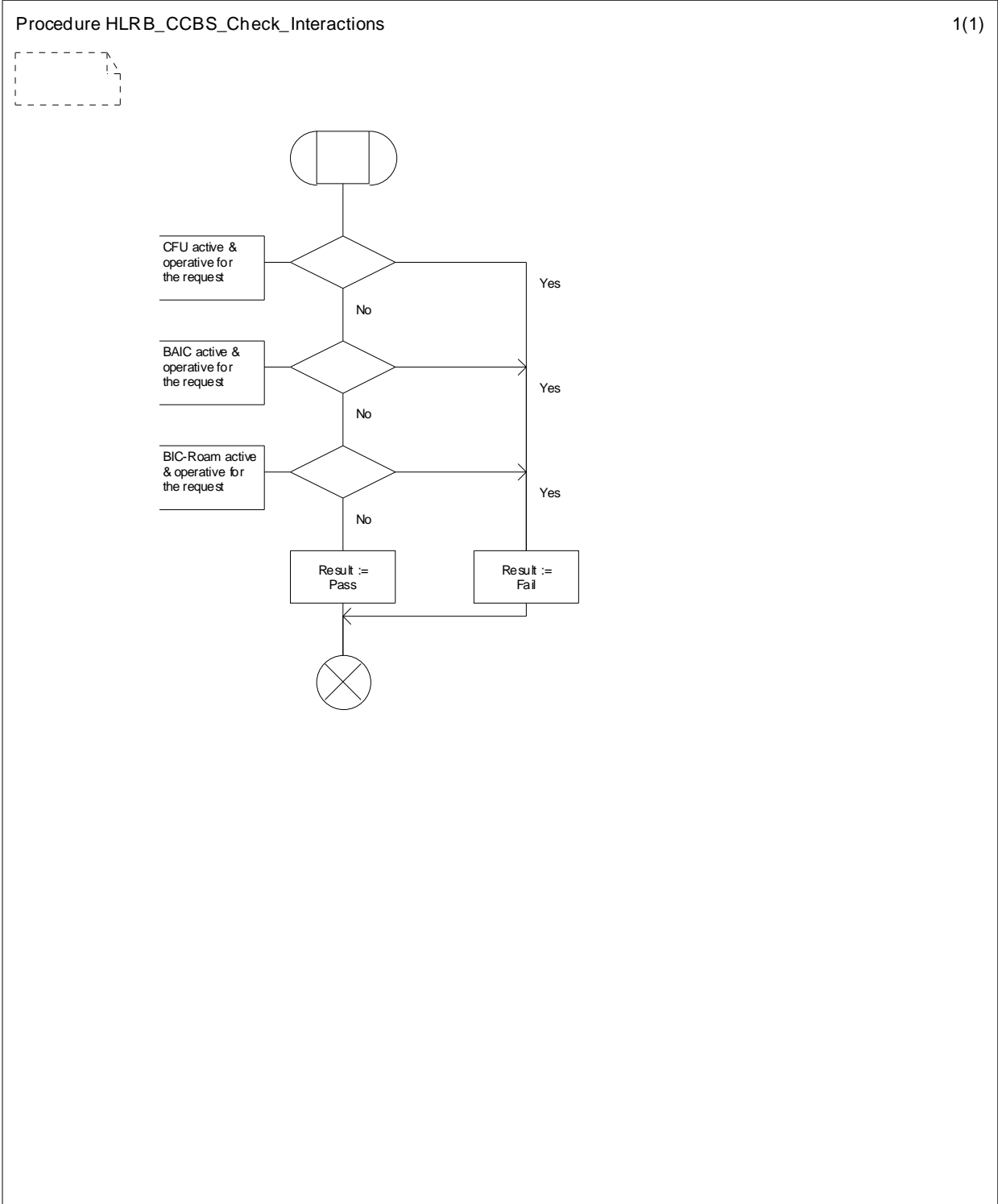
Figure 11.2.2.7: Procedure HLRB_Check_Interactions
