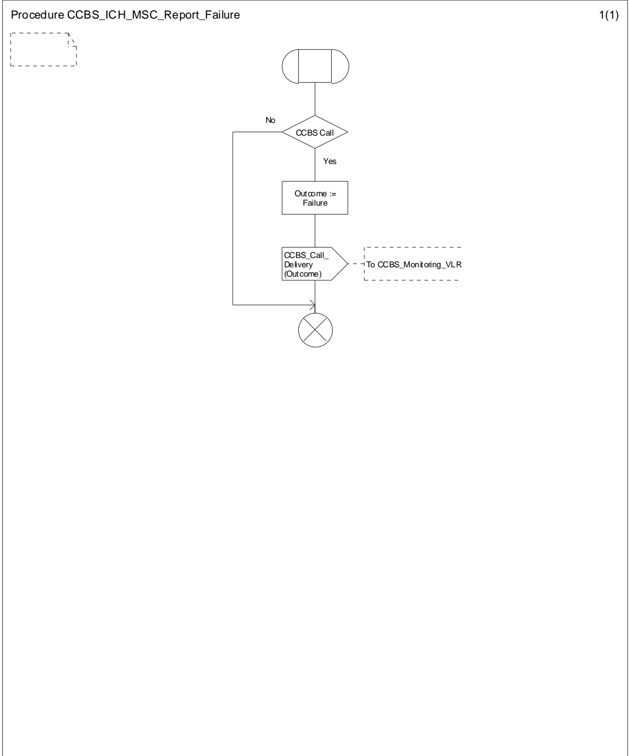
Figure 11.2.3.4: Procedure CCBS_ICH_MSC_Report_Failure
