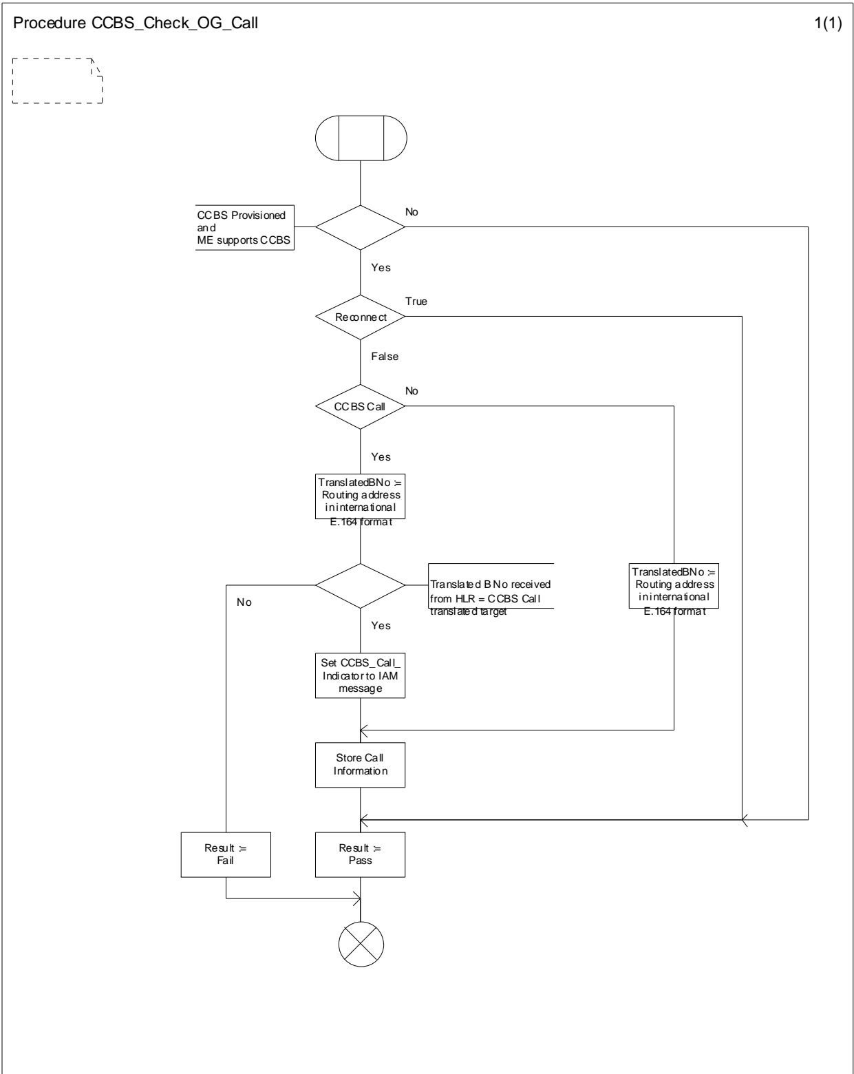
Figure 11.1.1.4: Procedure CCBS_Check_OG_Call
