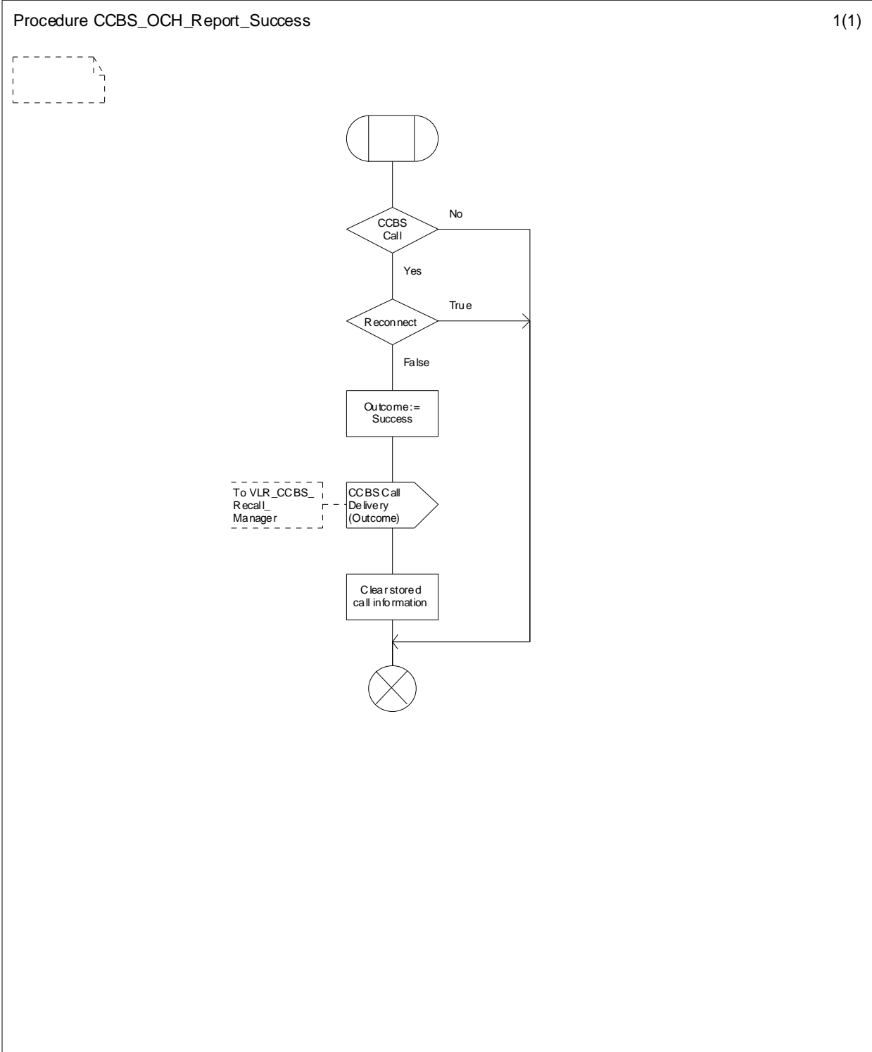
Figure 11.1.1.11: Procedure CCBS_OCH_Report_Success
