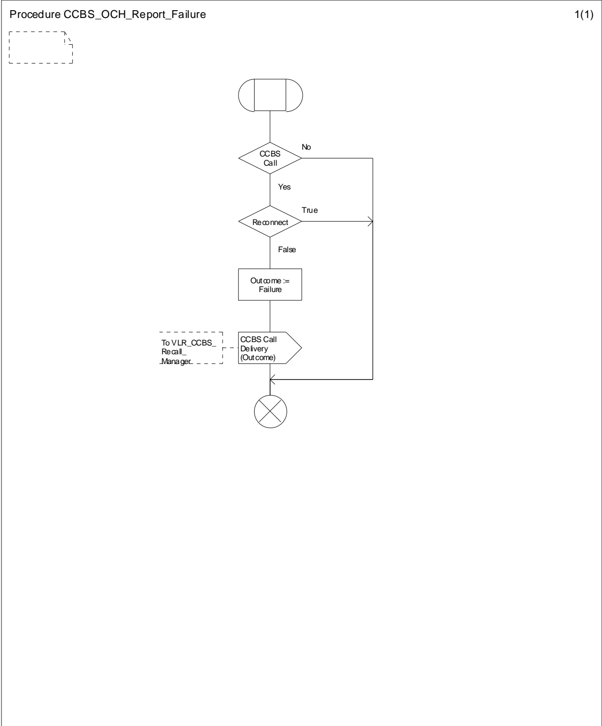
Figure 11.1.1.12: Procedure CCBS_OCH_Report_Failure
