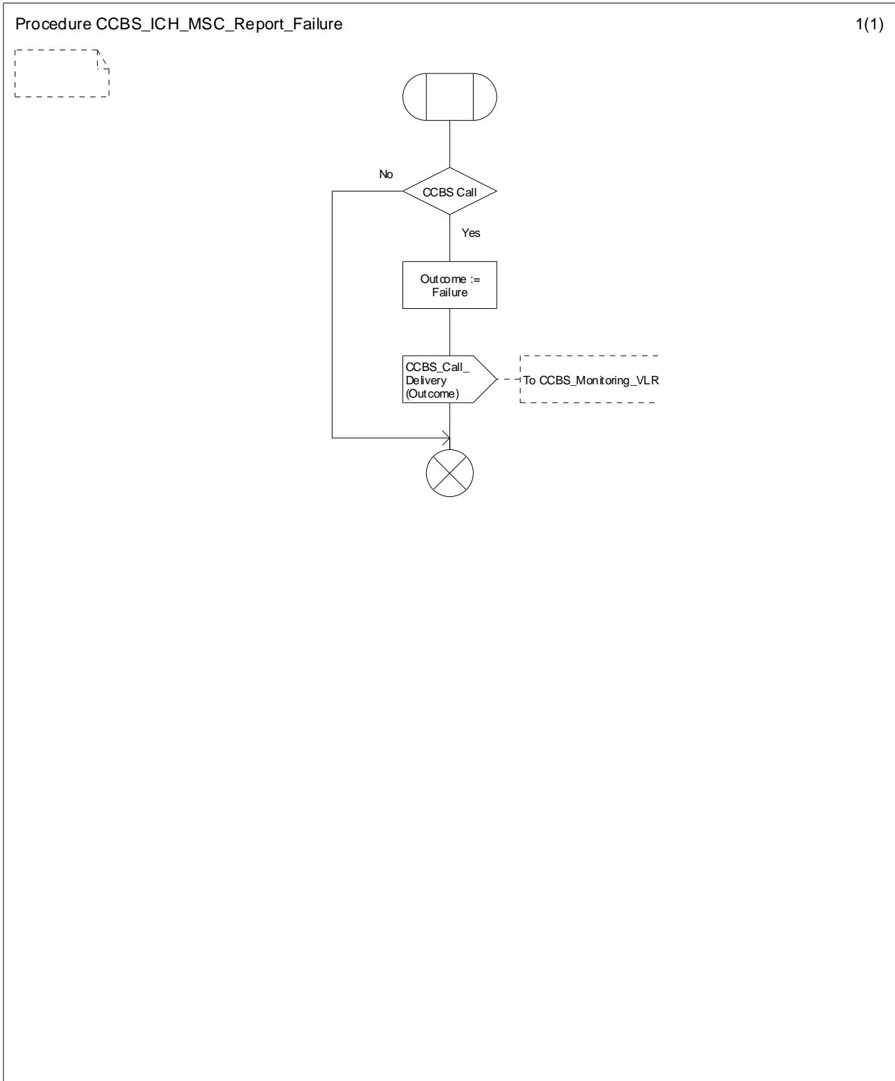
Figure 11.2.3.4: Procedure CCBS_ICH_MSC_Report_Failure
