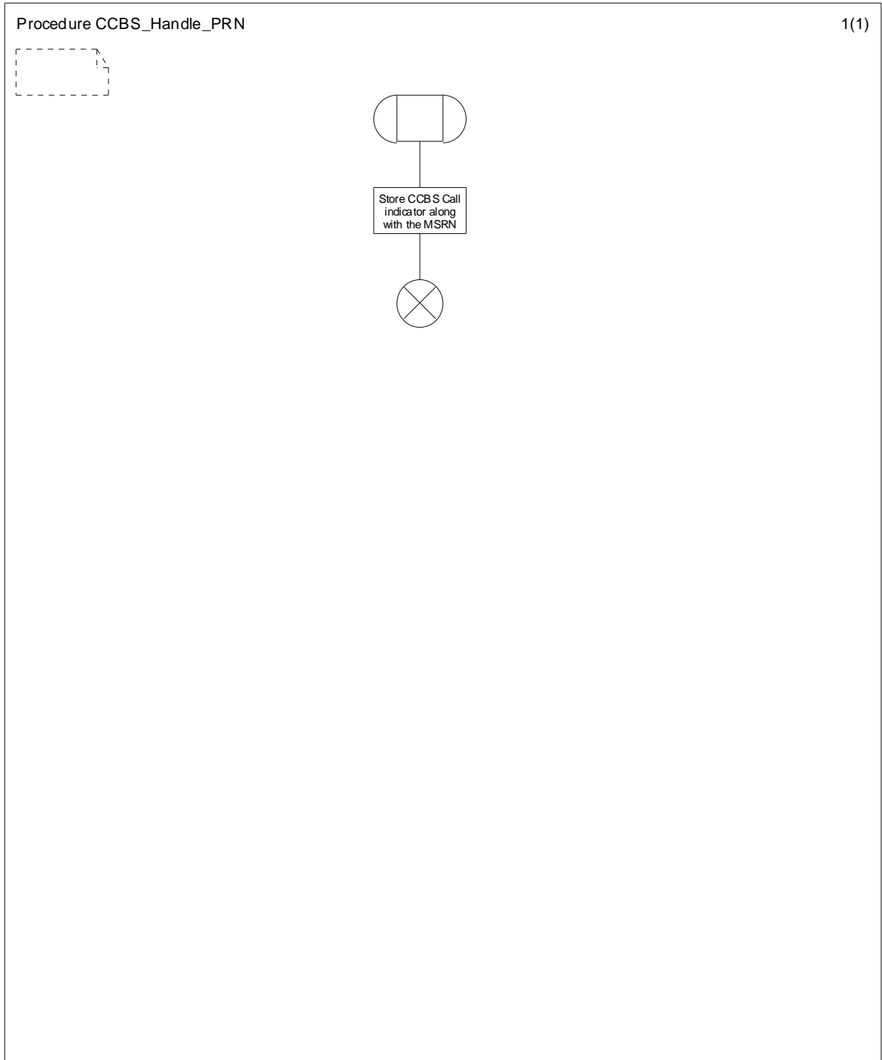
Figure 11.2.3.2: Procedure CCBS_Handle_PRN
