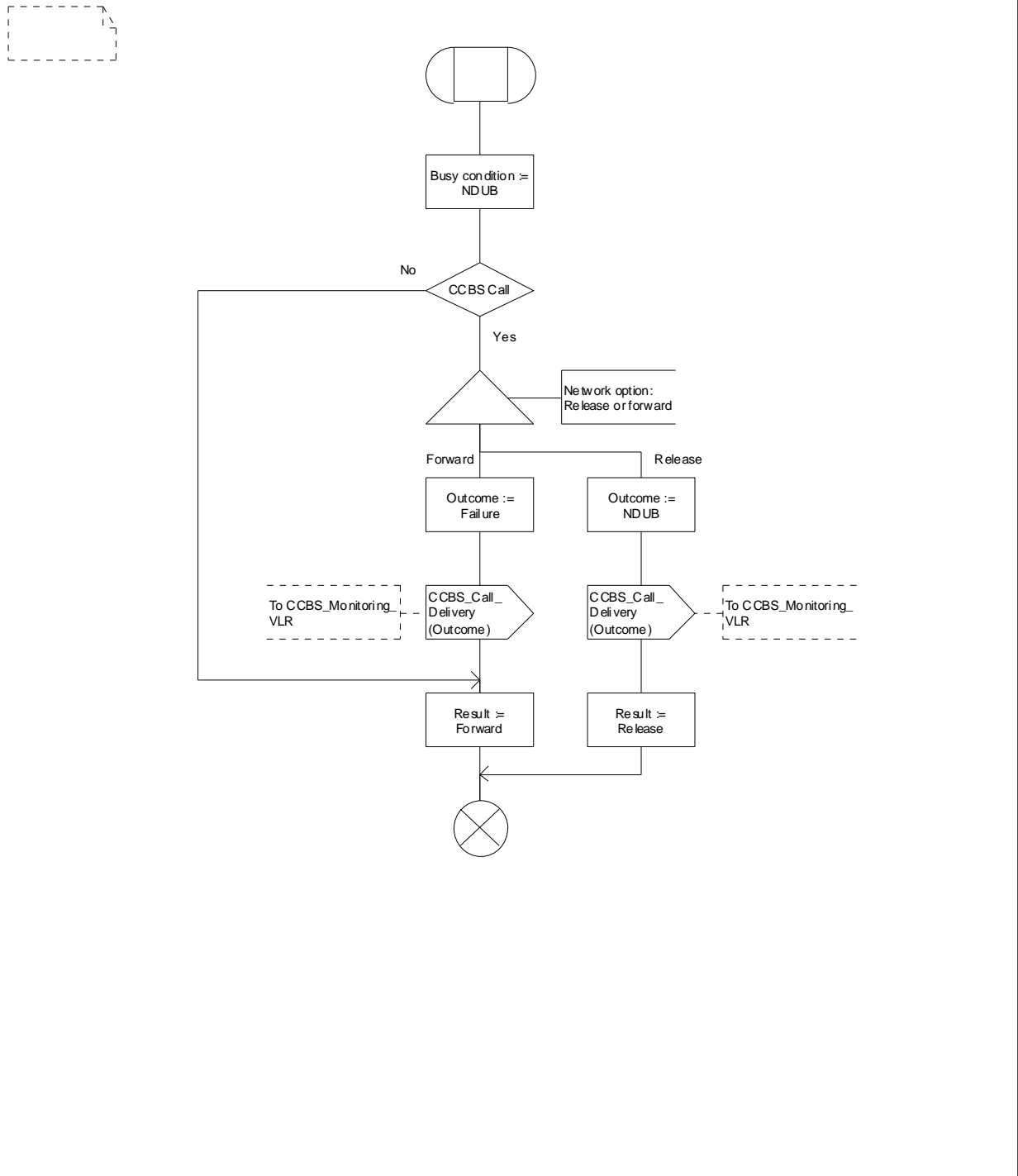
Figure 11.2.3.7: Procedure CCBS_ICH_Handle_NDUB
