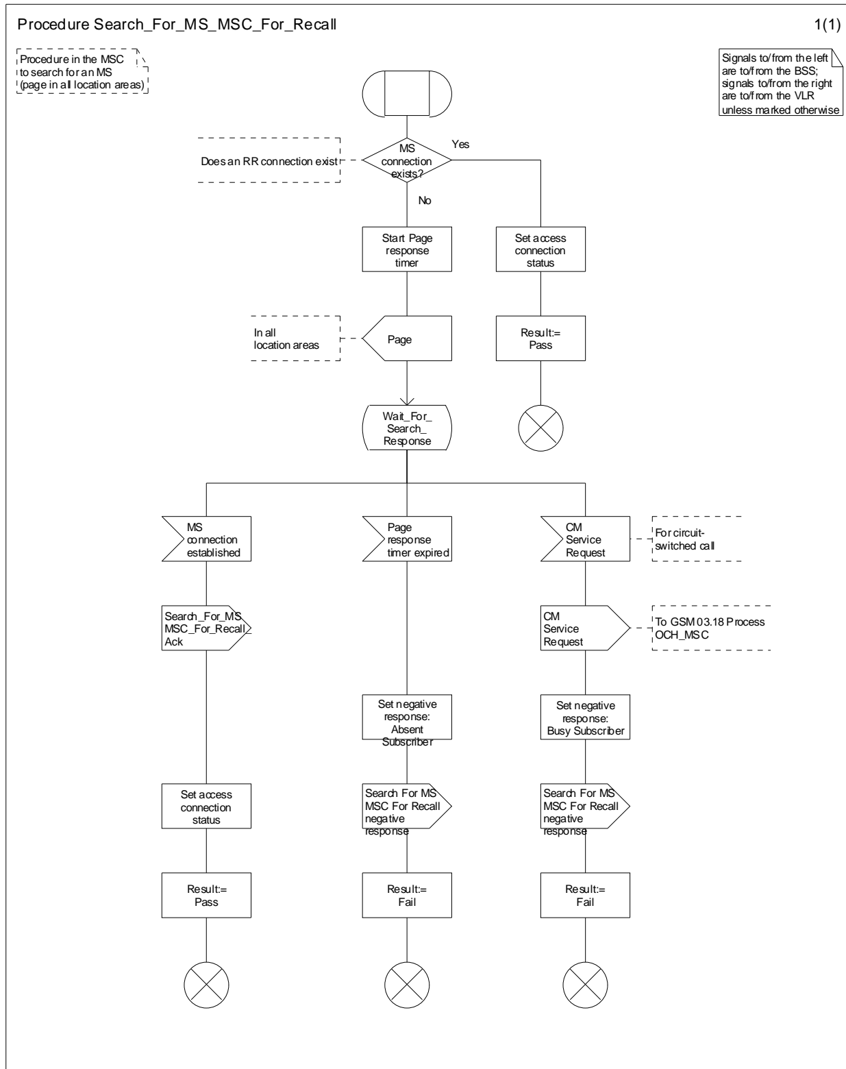
Figure 11.1.1.8: Procedure Search_For_MS_MSC_For_Recall
