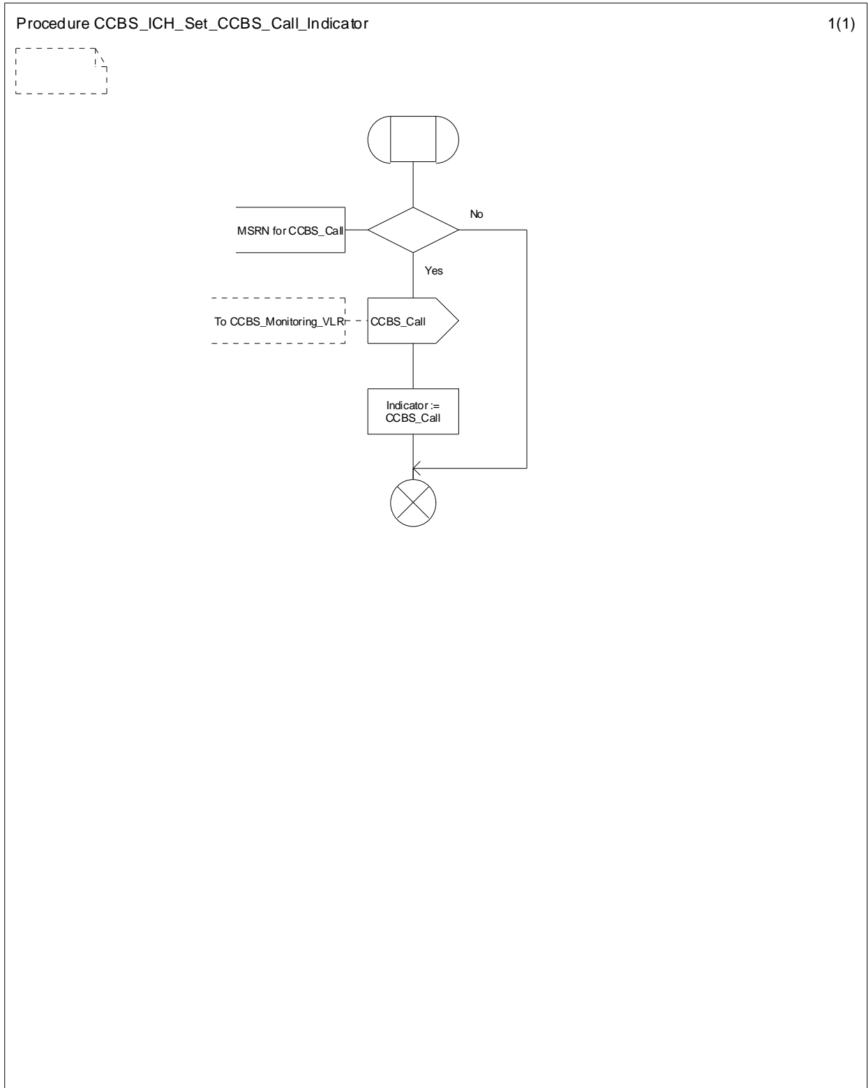
Figure 11.2.3.3: Procedure CCBS_ICH_Set_CCBS_Call_Indicator
