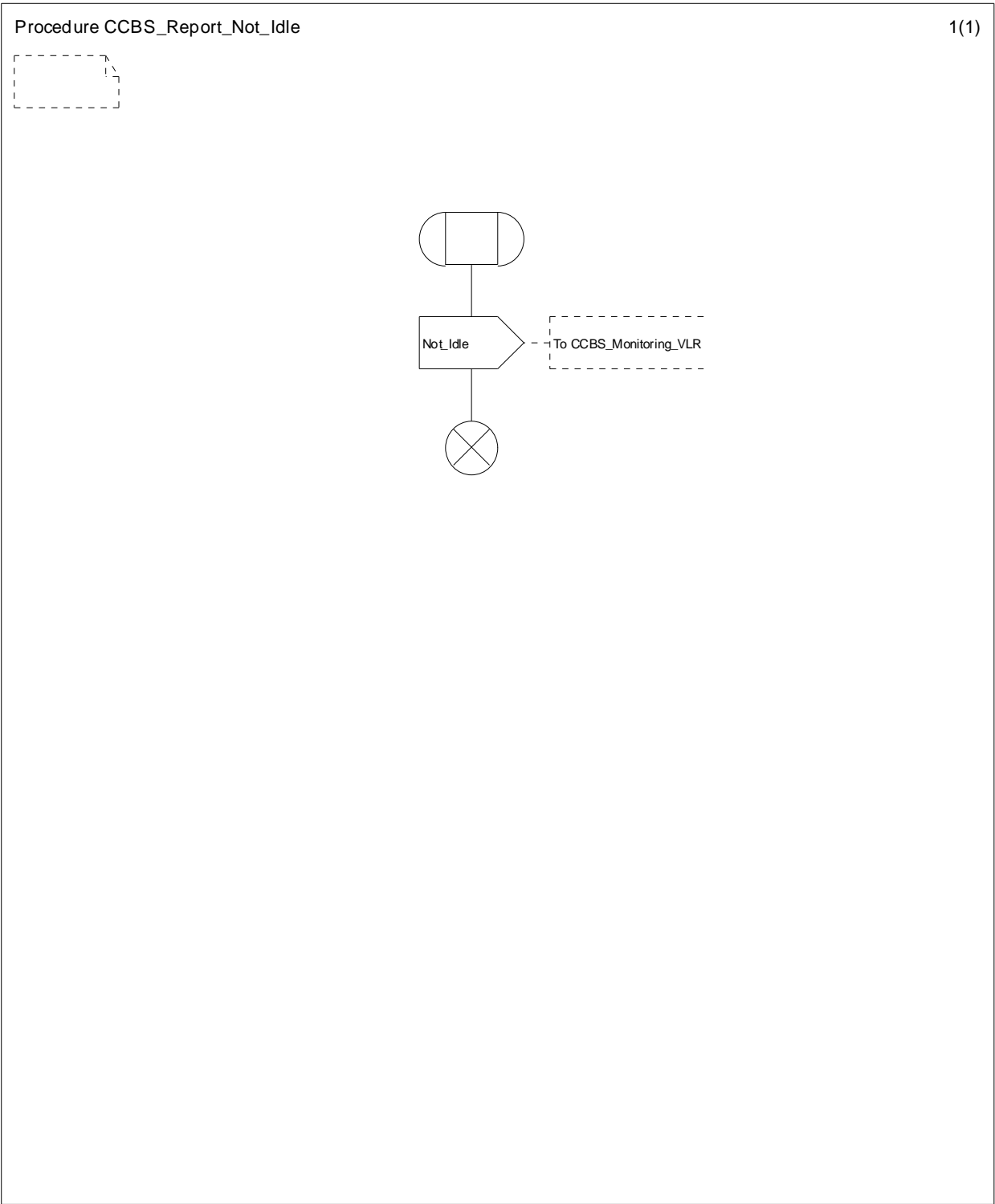
Figure 11.3.5: Procedure CCBS_Report_Not_Idle
