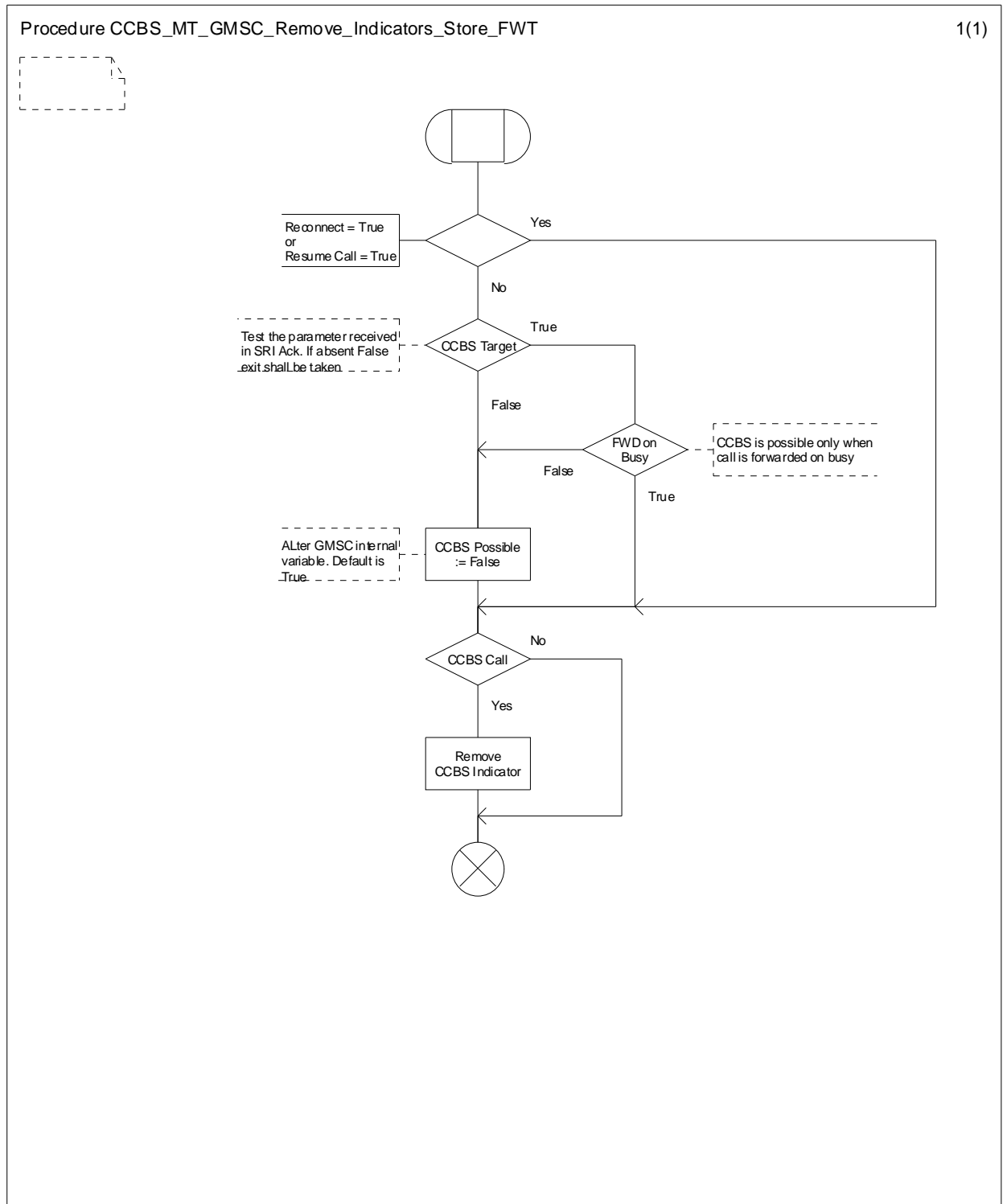
Figure 11.2.1.3: Procedure CCBS_MT_GMSC_Remove_Indicators_Store_FWT
