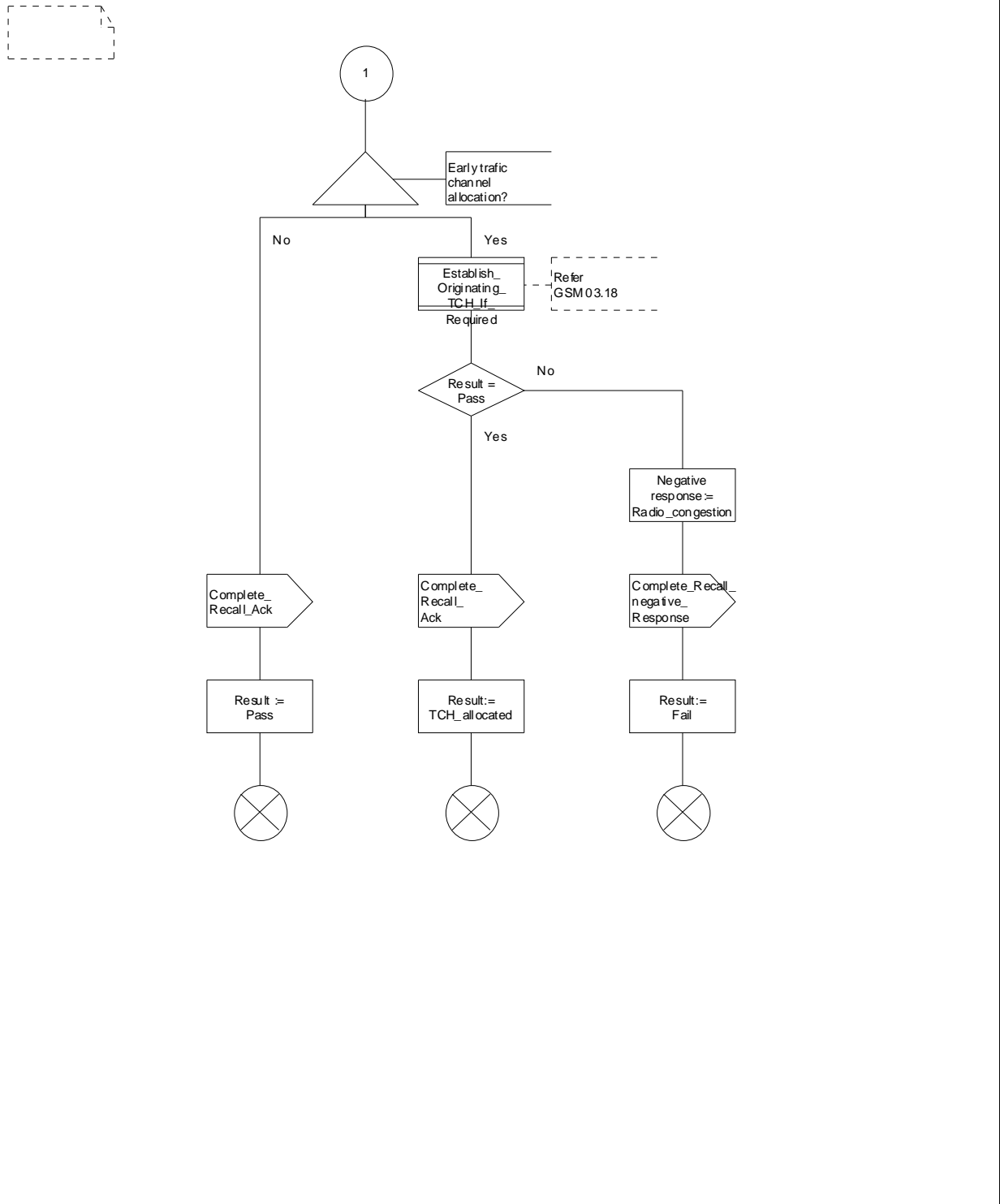
Figure 11.1.1.10: Procedure Complete_Recall_MSC (sheet 2 of 2)
