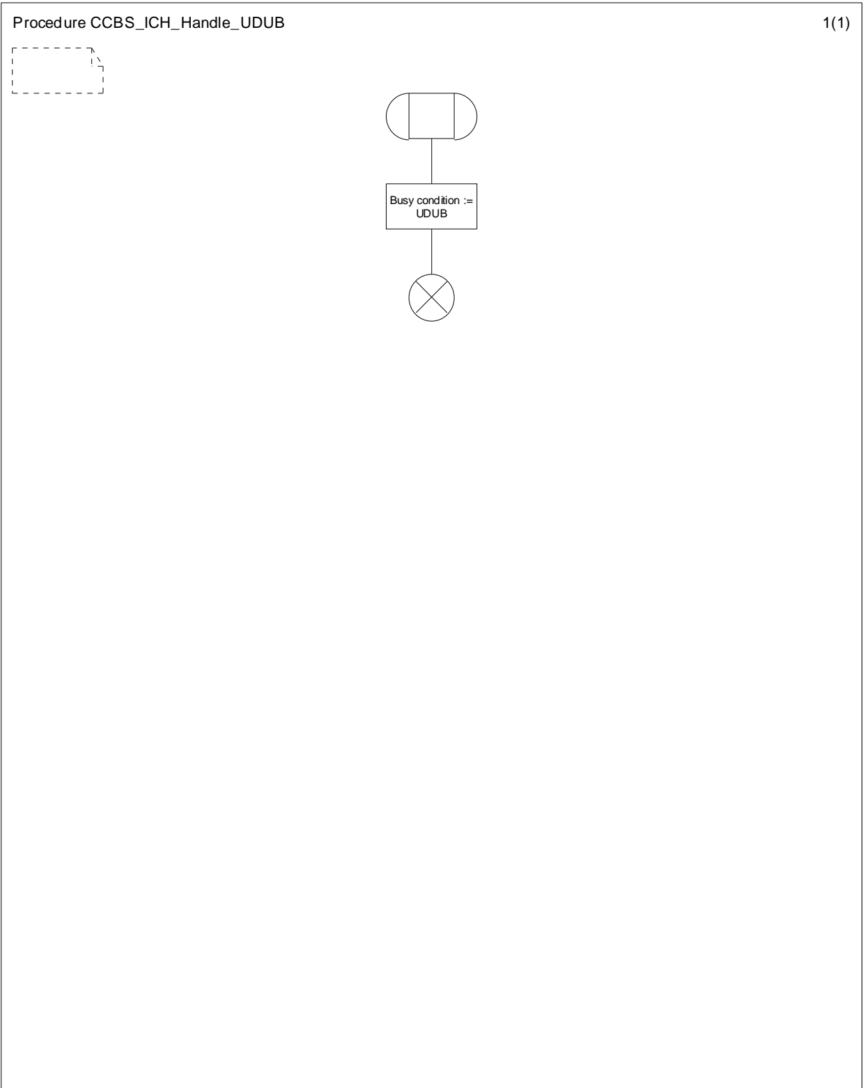
Figure 11.2.3.8: Procedure CCBS_ICH_Handle_UDUB
