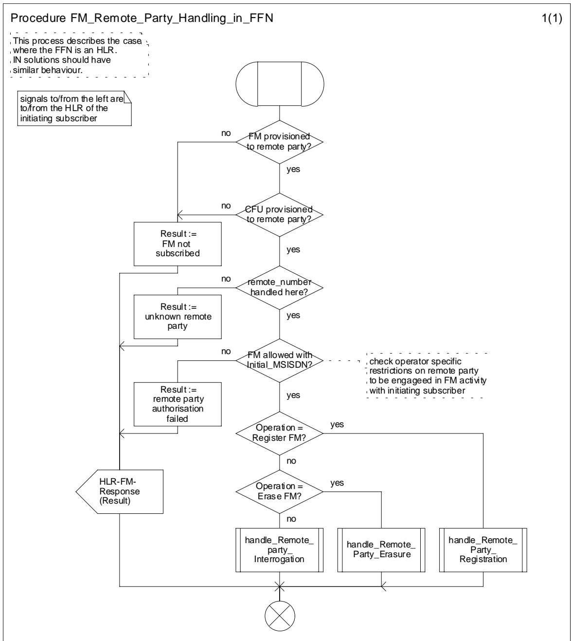
Figure 4.5: Procedure: FM_Remote_Party_Handling_in_FFN
