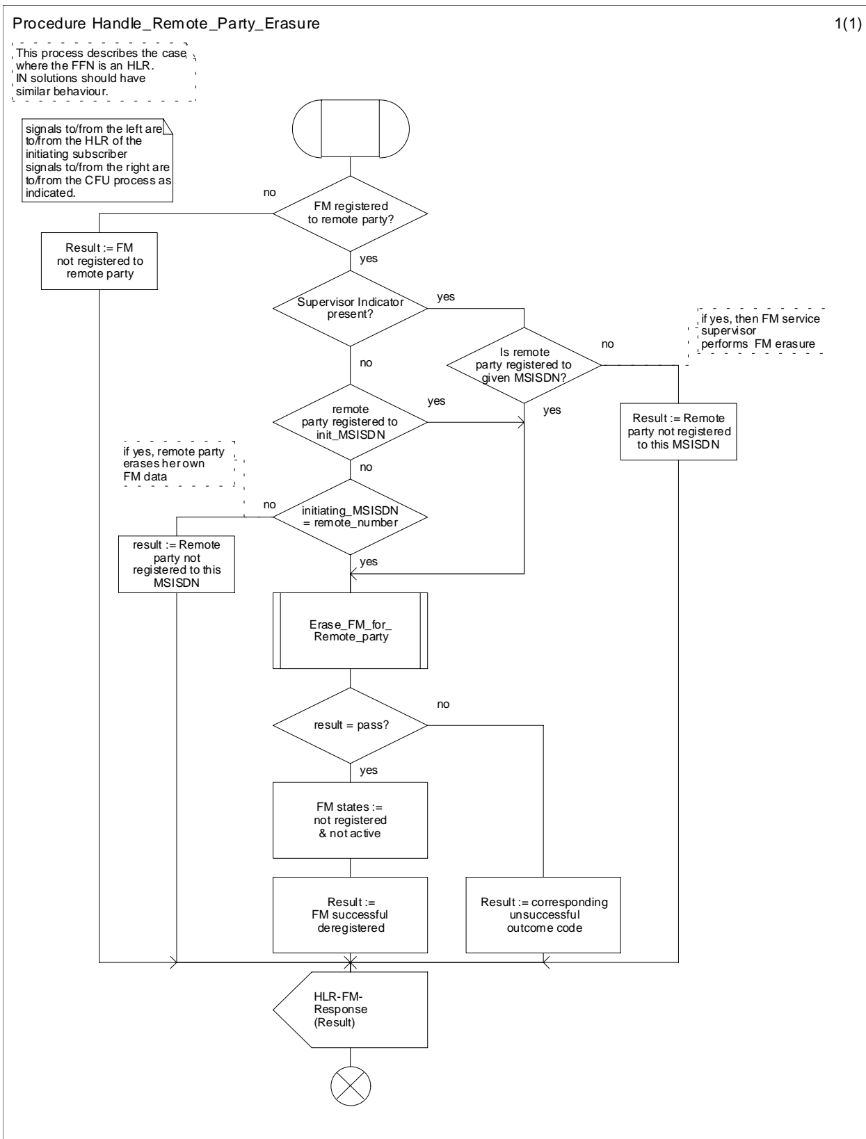
Figure 4.7: Procedure: Handle_Remote_Party_Erasure
