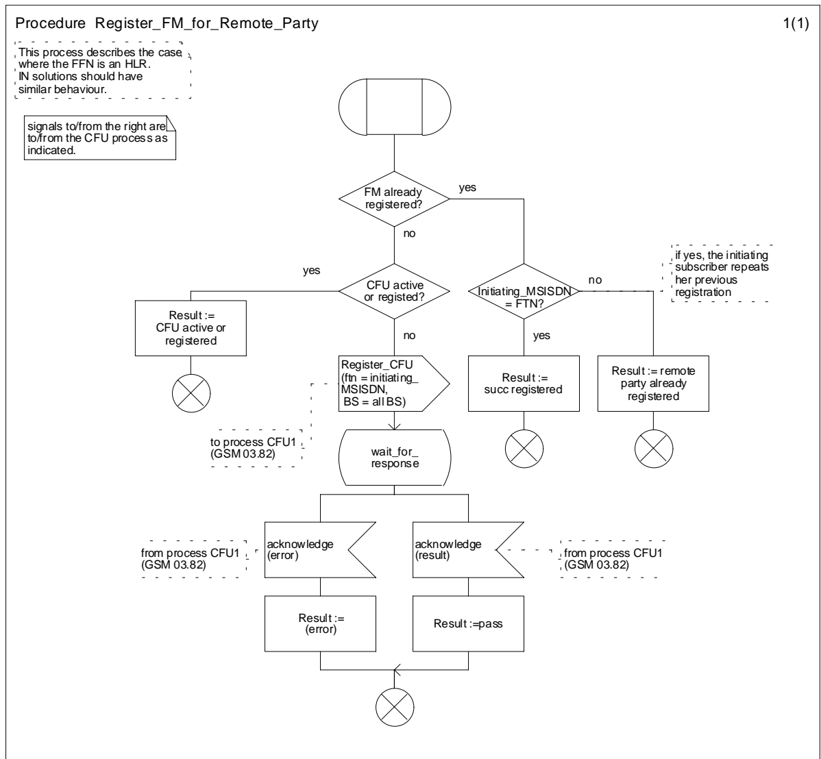
Figure 4.6a: Procedure Register_FM_for_Remote_Party
