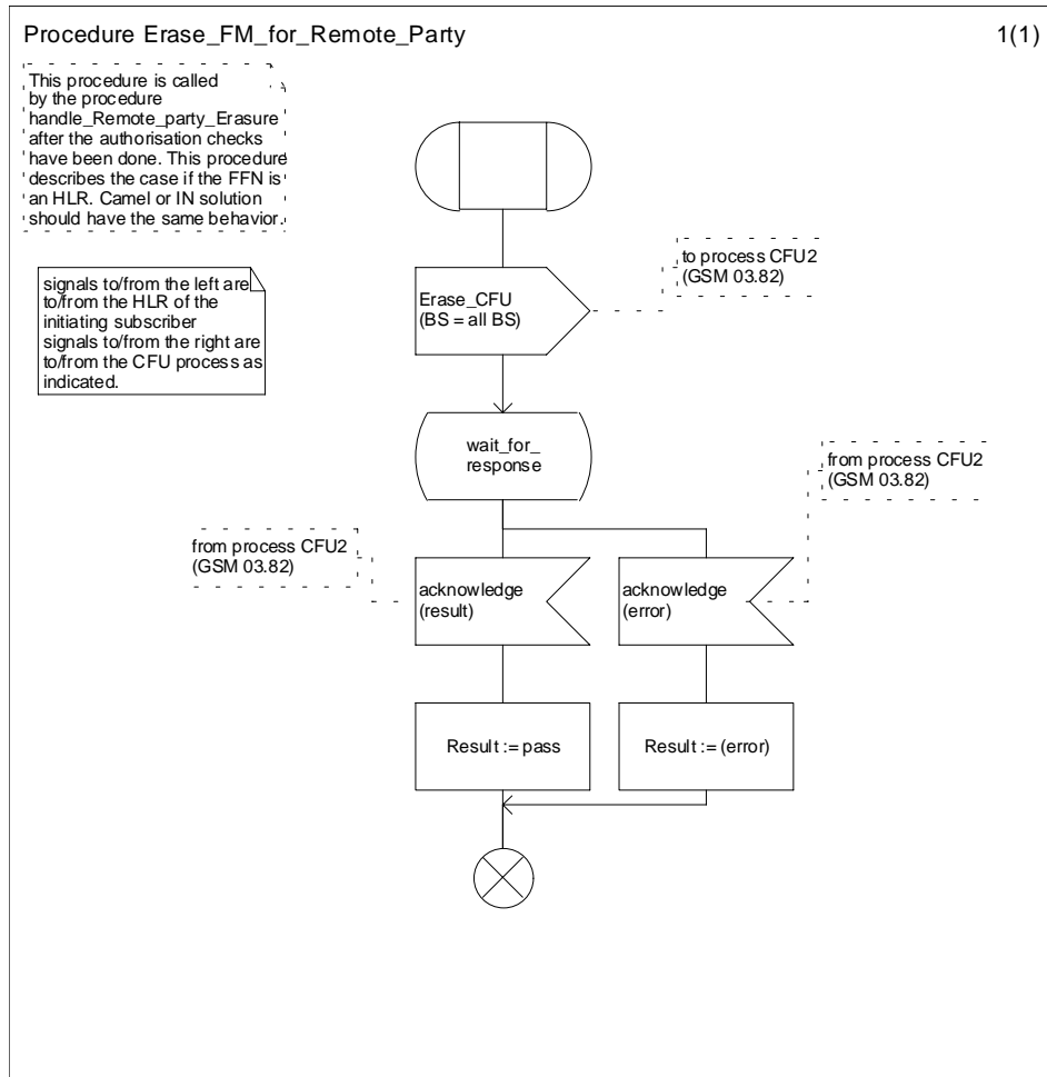
Figure 4.7a: Procedure Erase_FM_for_Remote_party
