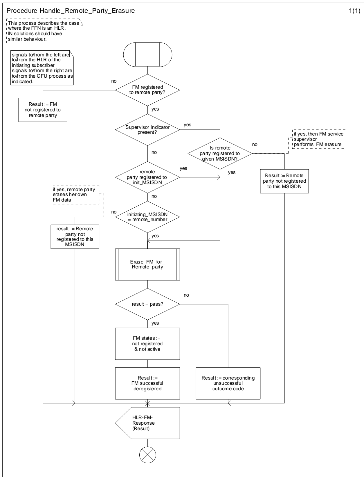
Figure 4.7: Procedure: Handle_Remote_Party_Erasure
