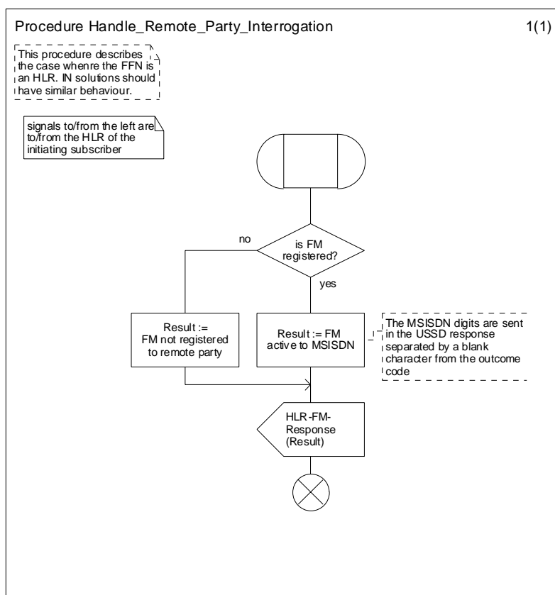
Figure 4.8: Procedure Handle_Remote_Party_Interrogation
