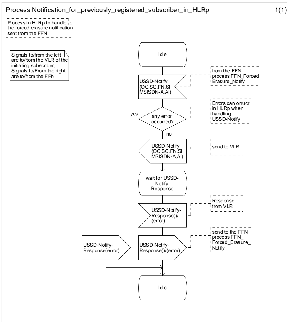
Figure 4.2a: Process Notification_for_previously_registered_subscriber_in_HLRp
