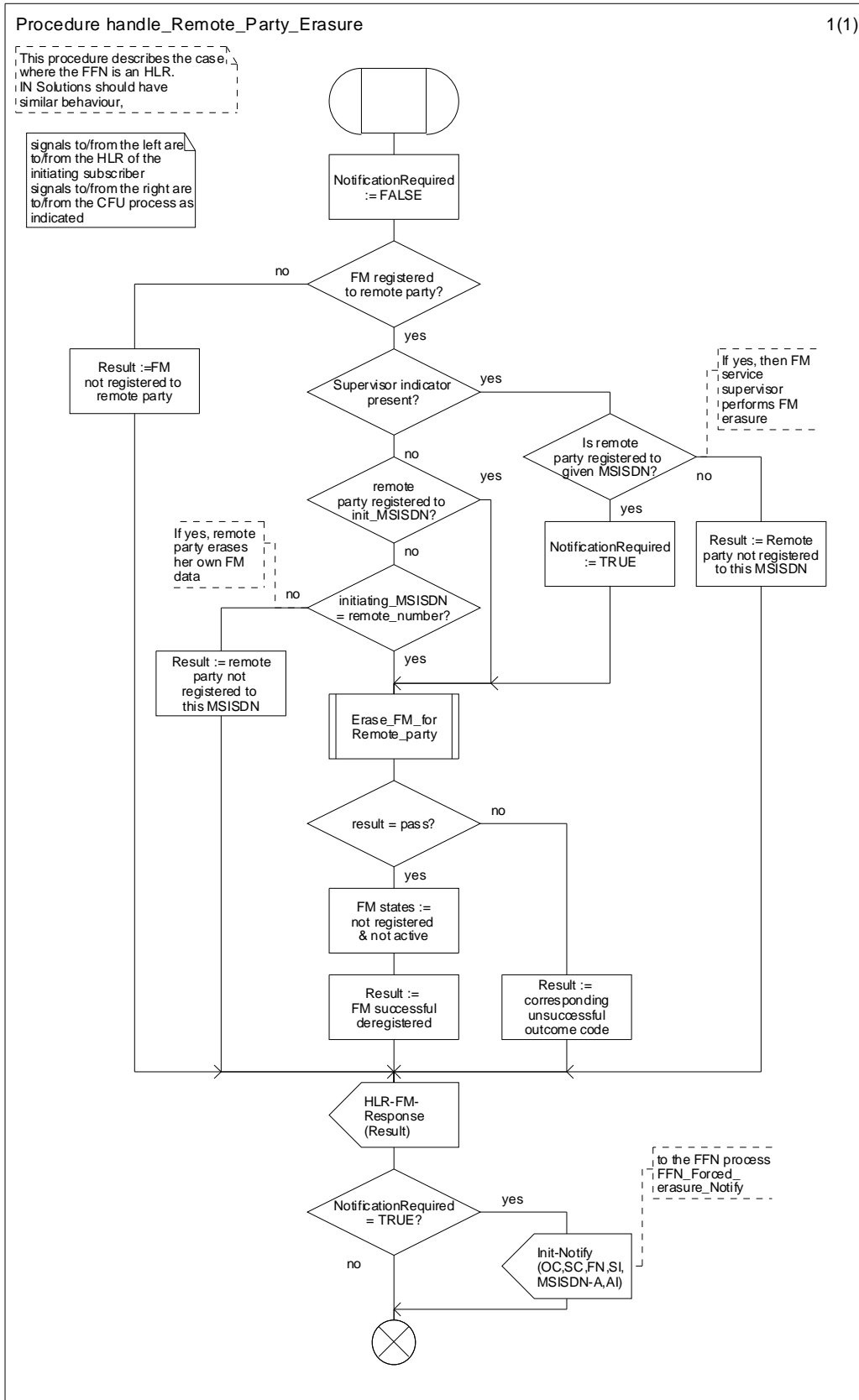
Figure 4.7: Procedure: Handle_Remote_Party_Erasure
