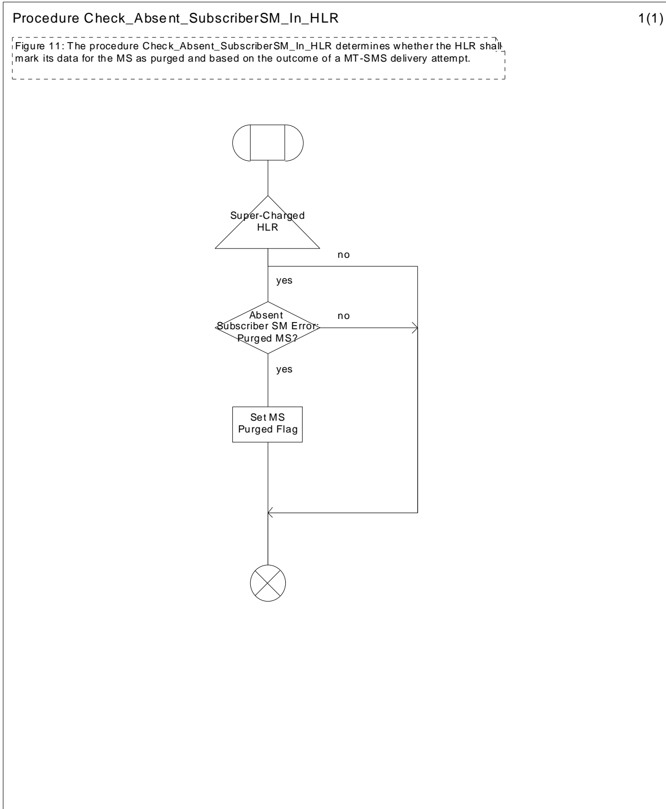
Figure 11: Procedure Check_Absent_SubscriberSM_In_HLR
