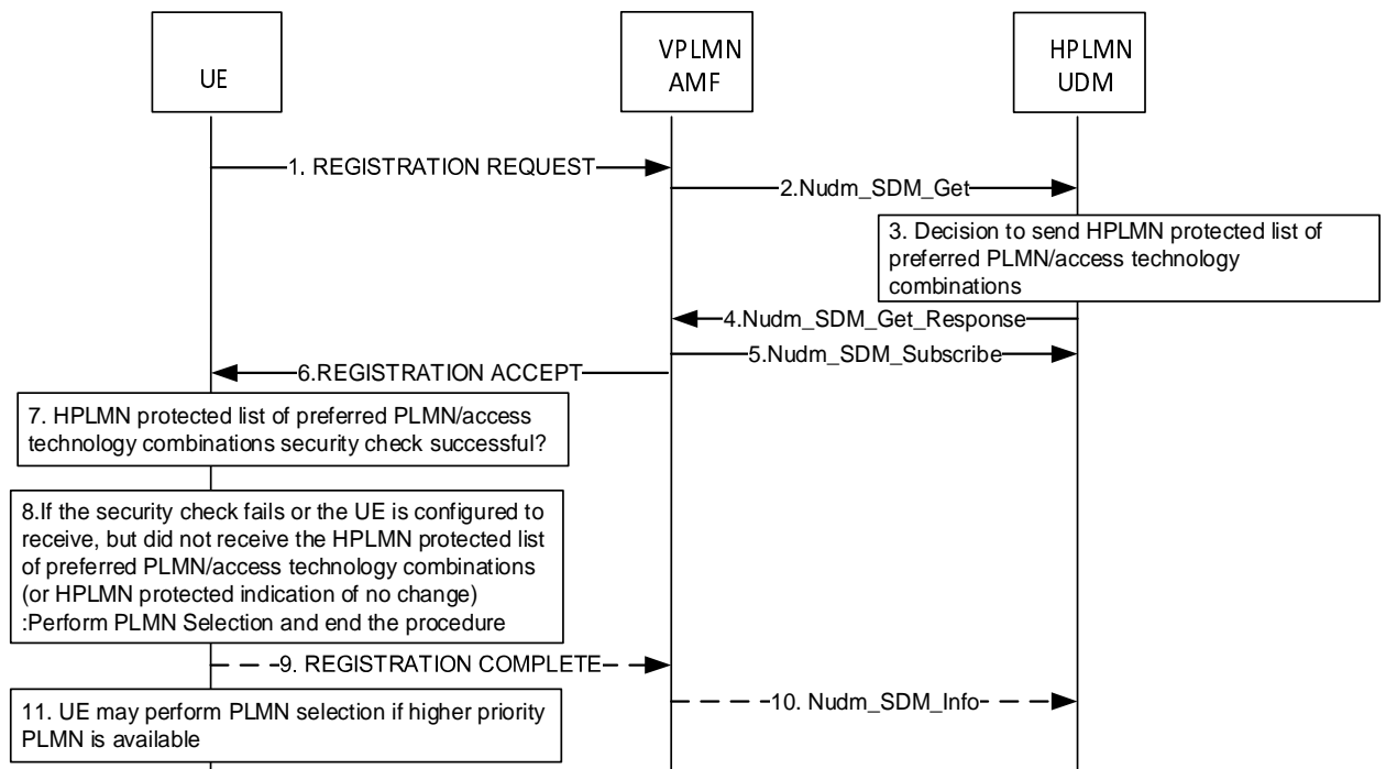
Figure C.2.1: Procedure for providing list of preferred PLMN/access technology combinations
