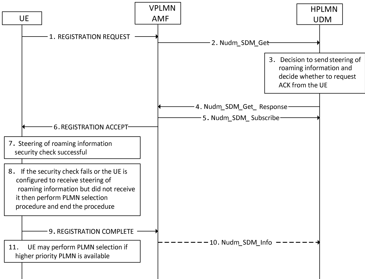
Figure C.2.1: Procedure for providing list of preferred PLMN/access technology combinations
