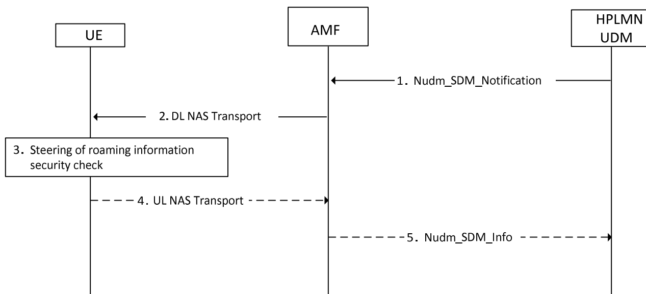
Figure C.3.1: Procedure for providing list of preferred PLMN/access technology combinations after registration
