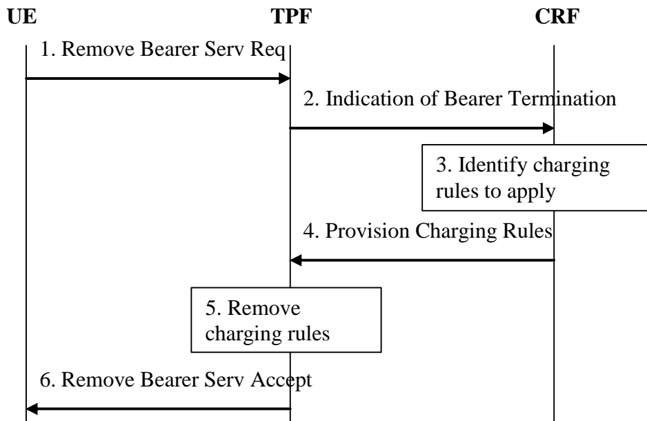
Figure 7.3: Bearer Service Termination in case of offline charging
