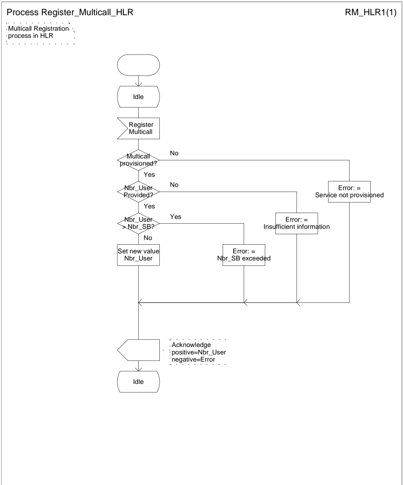
Figure 2: Process Register_Multicall_HLR
