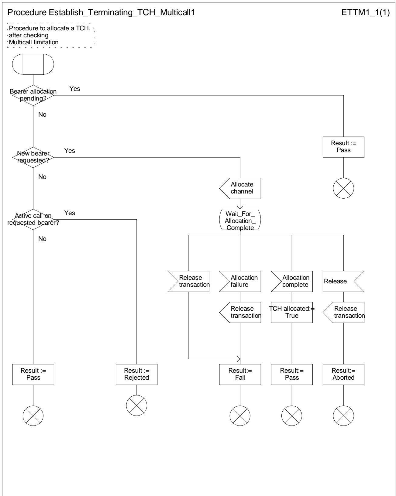
Figure 11: Procedure Establish_Terminating_TCH_Multicall1
