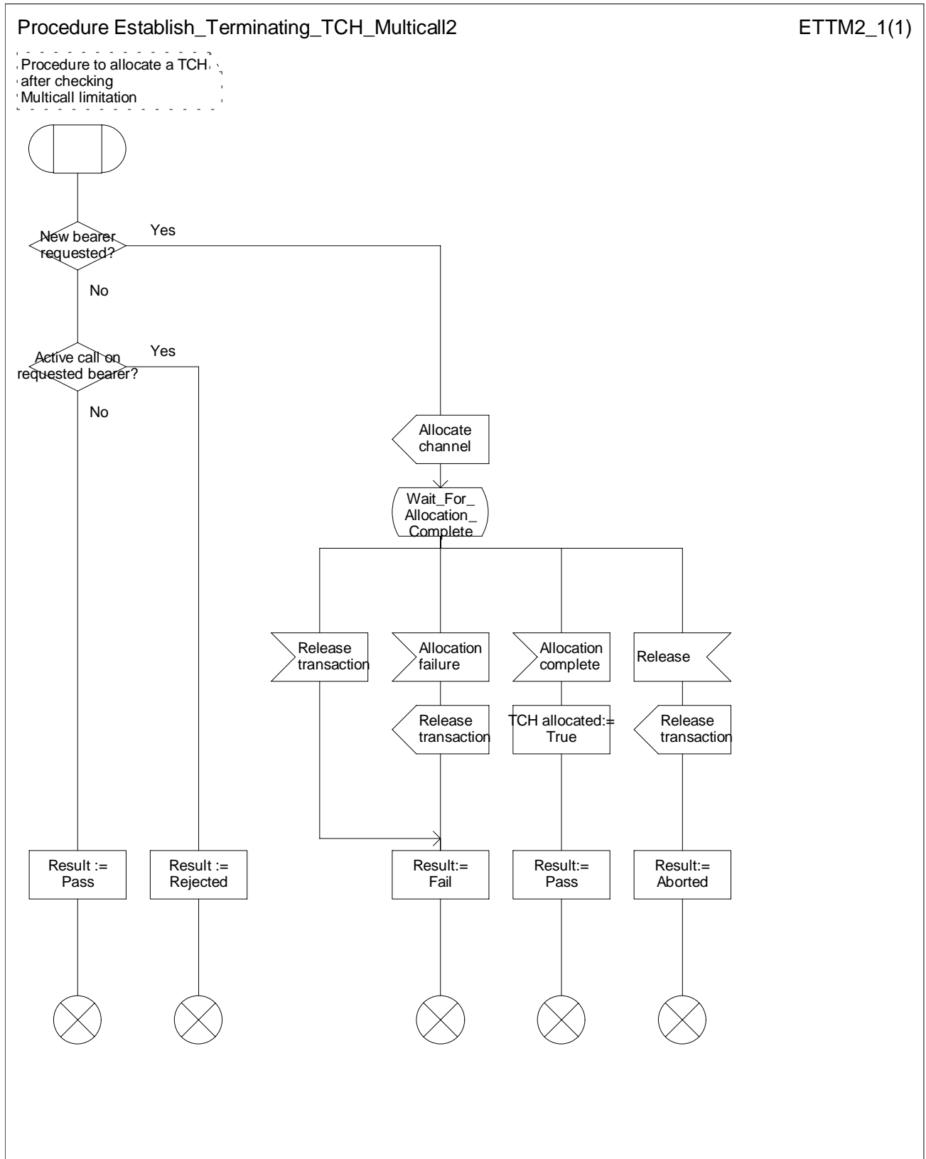
Figure 12: Procedure Establish_Terminating_TCH_Multicall2
