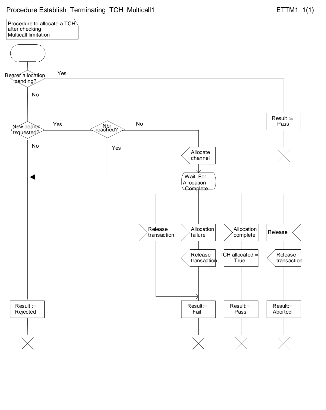
Figure 11: Procedure Establish_Terminating_TCH_Multicall1
