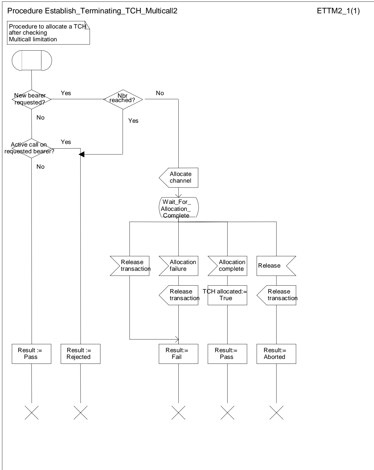
Figure 12: Procedure Establish_Terminating_TCH_Multicall2
