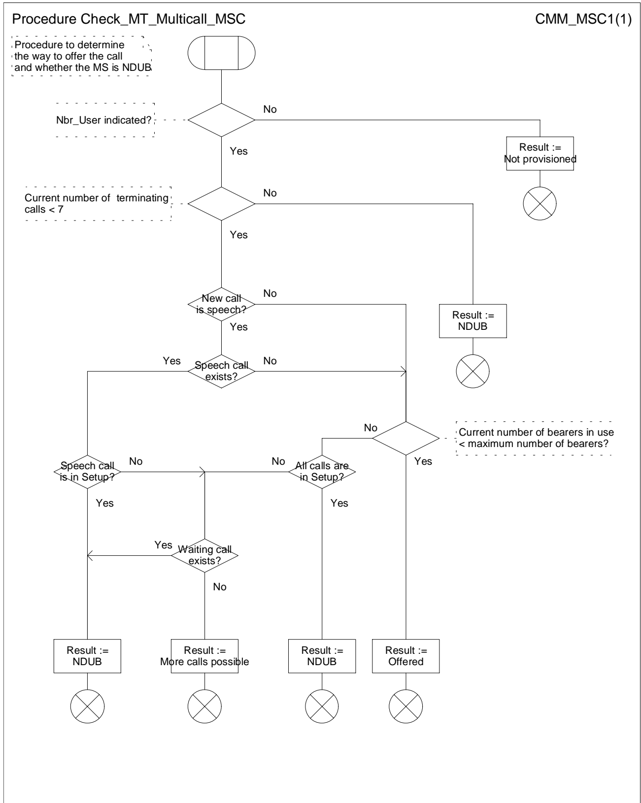
Figure 10: Procedure Check_MT_Multicall_MSC
