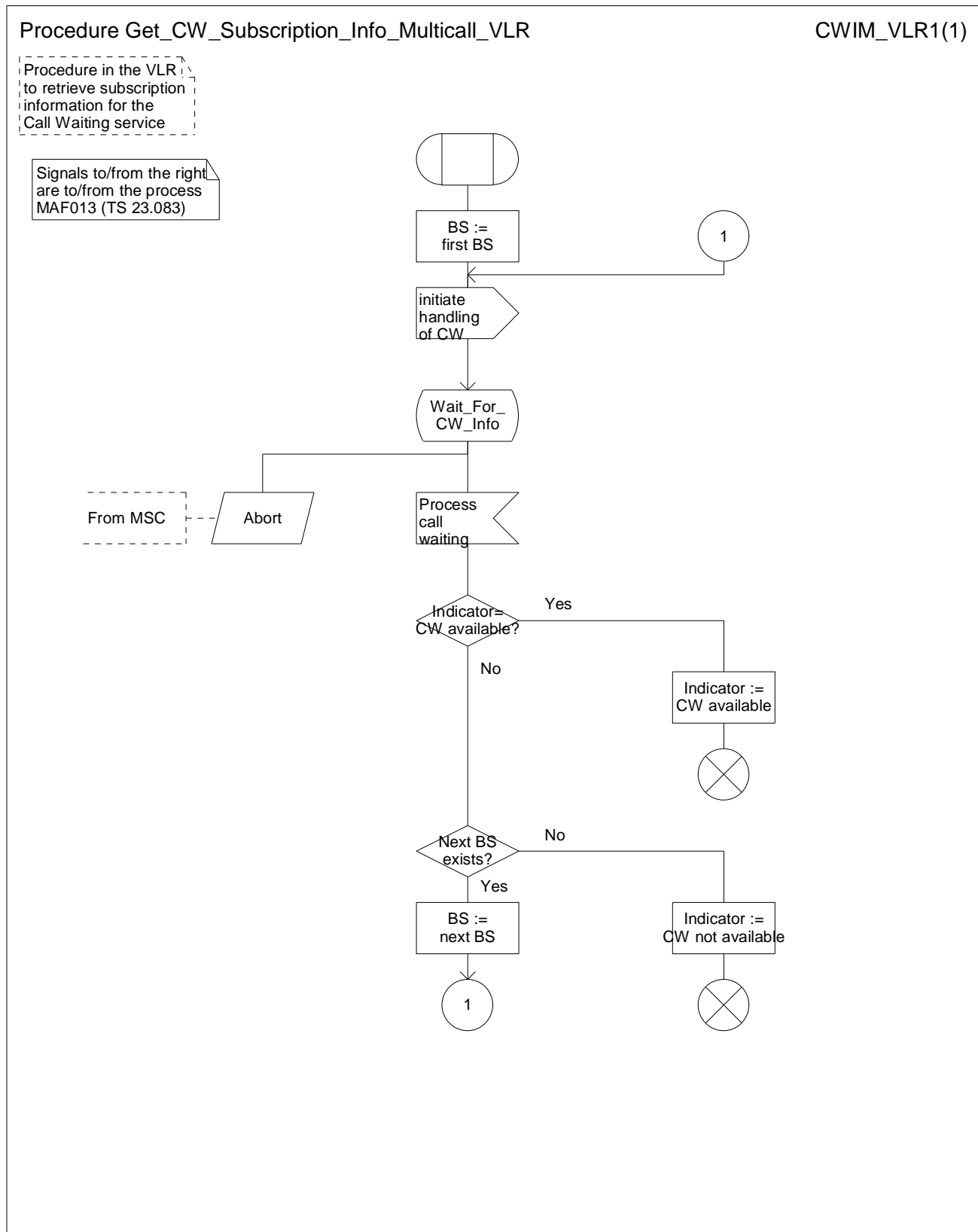
Figure 13: Procedure Get_CW_Subscription_Info_Multicall_VLR
