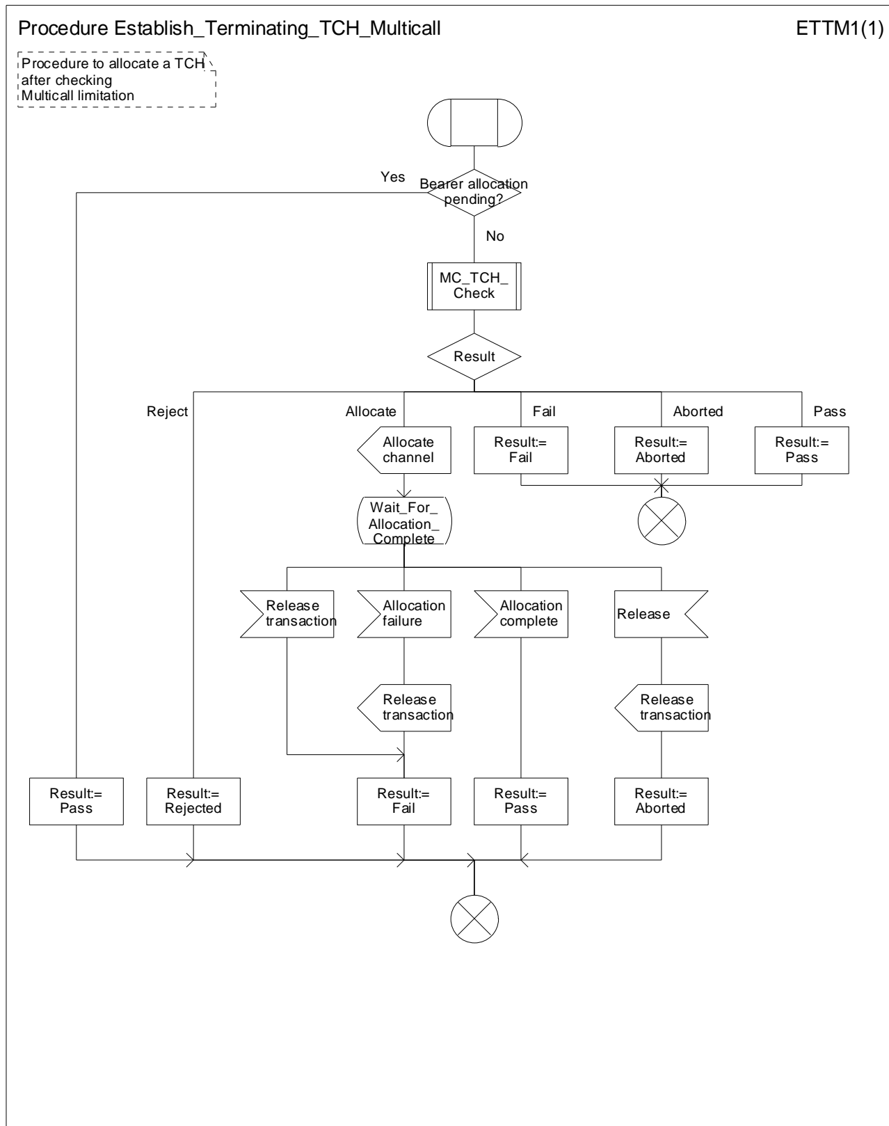
Figure 11: Procedure Establish_Terminating_TCH_Multicall
