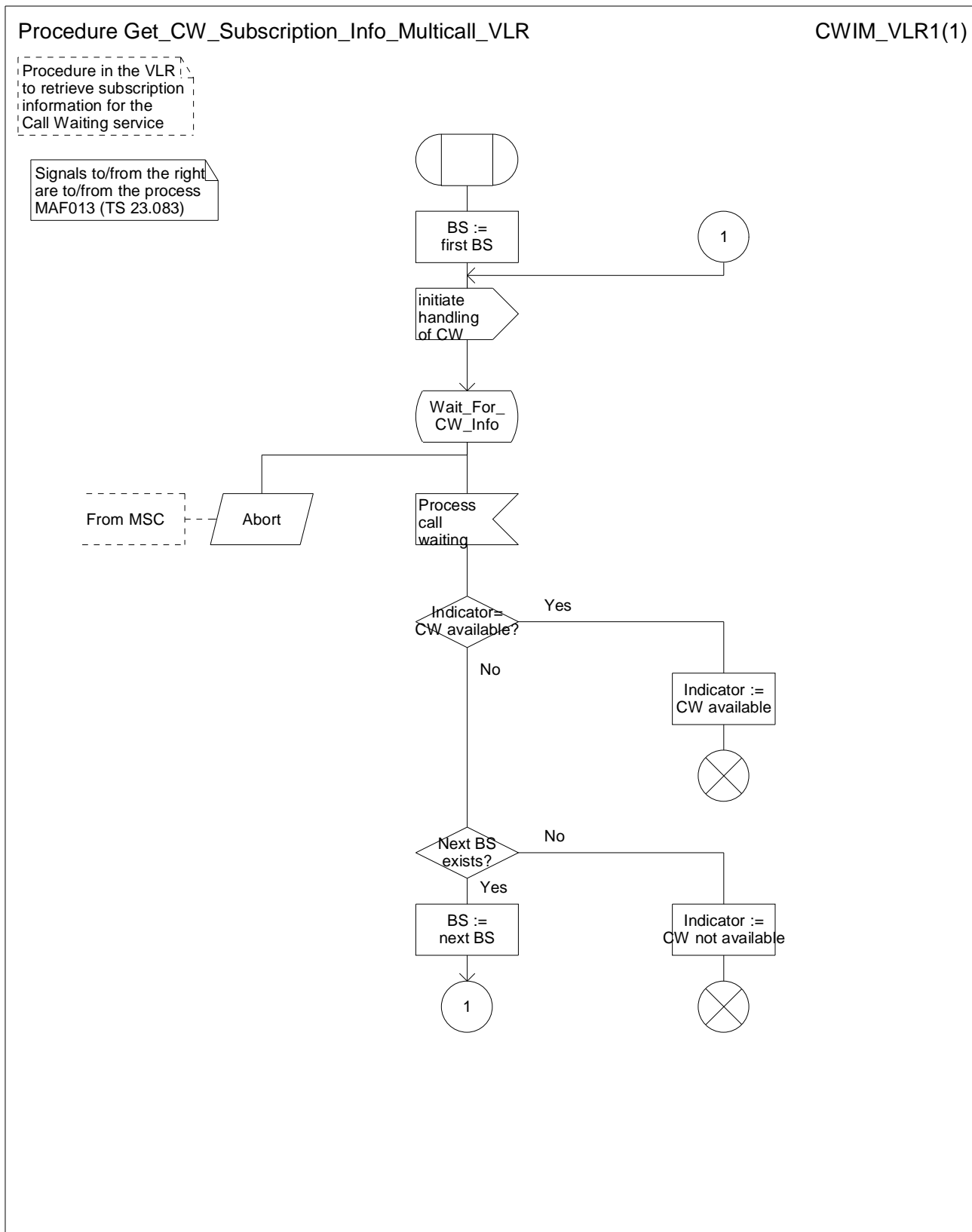
Figure 13: Procedure Get_CW_Subscription_Info_Multicall_VLR
