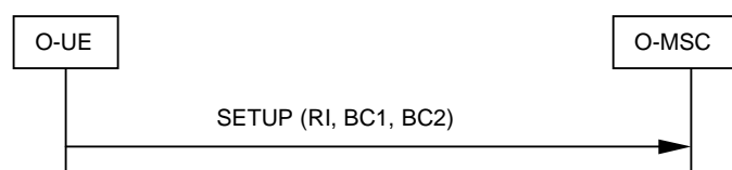
Figure 4.1: SETUP message towards the originating MSC
