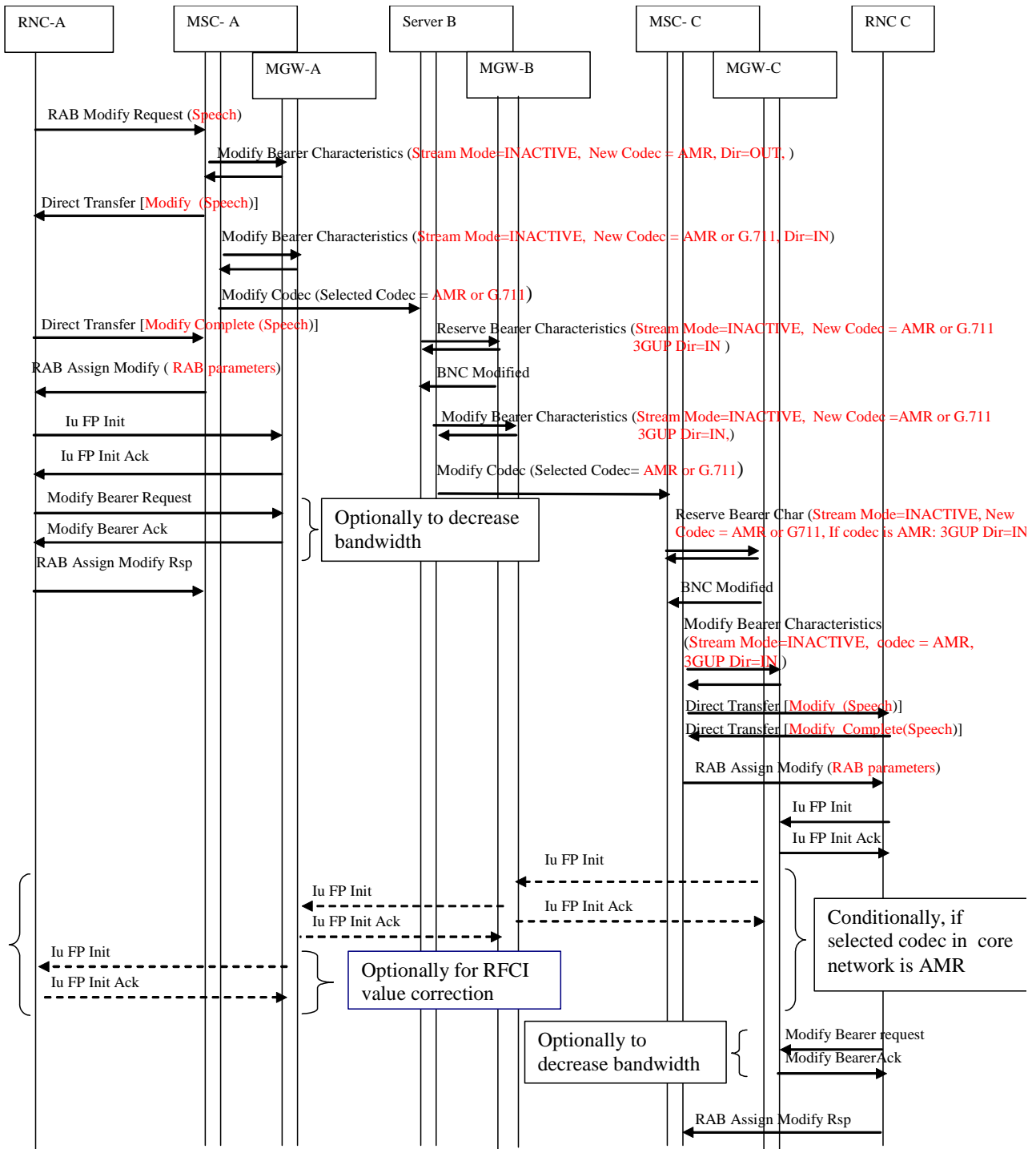
Figure 4.3.5.1/7: Network-initiated service change from MuMe to speech
