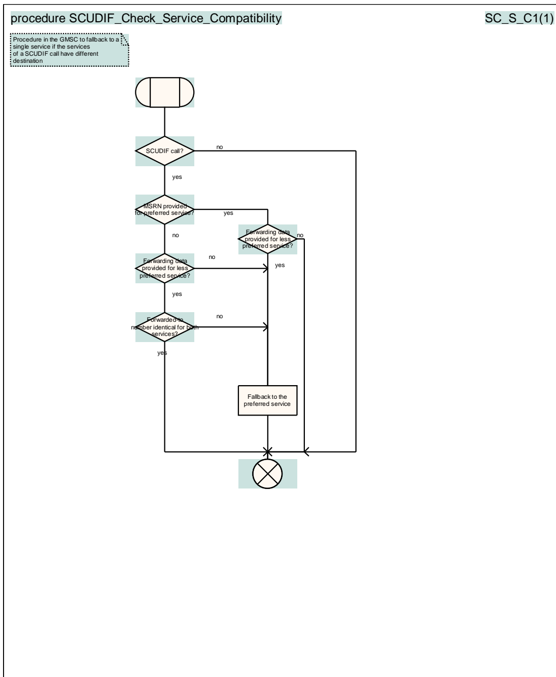
Figure 4.16K: Procedure SCUDIF_Check_Service_Compatibility
