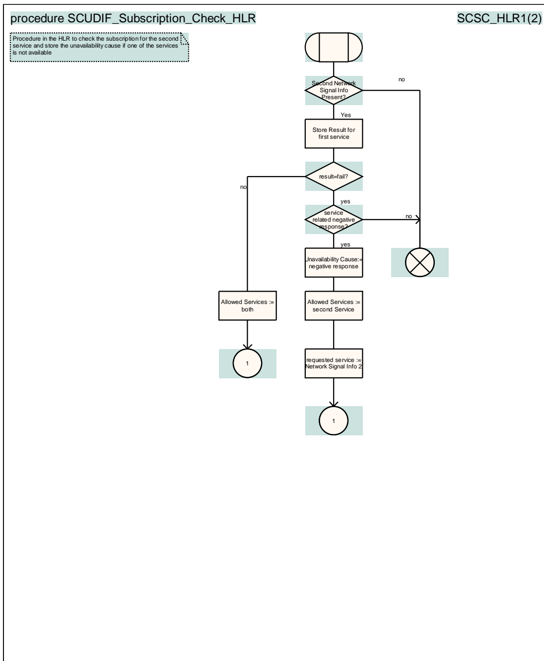
Figure 4.16A: Procedure SCUDIF_Subscription_Check_HLR (sheet 1)
