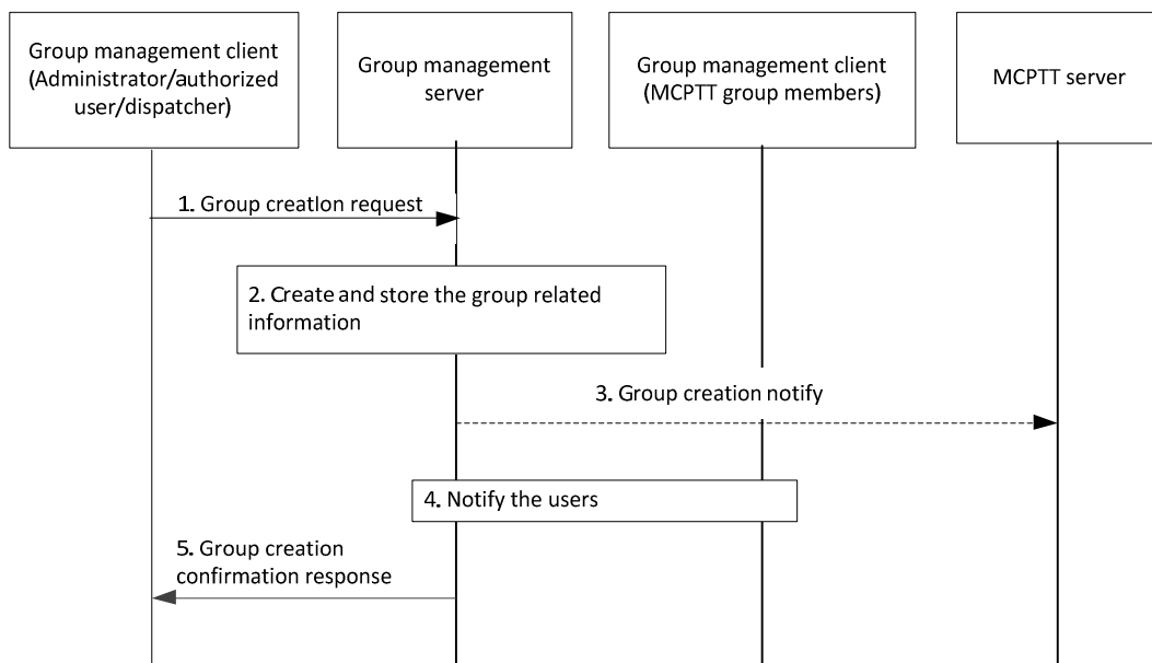
Figure 10.4.3-1: Group creation
