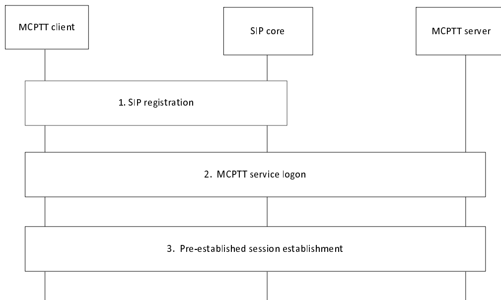
Figure 10.5.3.1-1: Pre-established session
