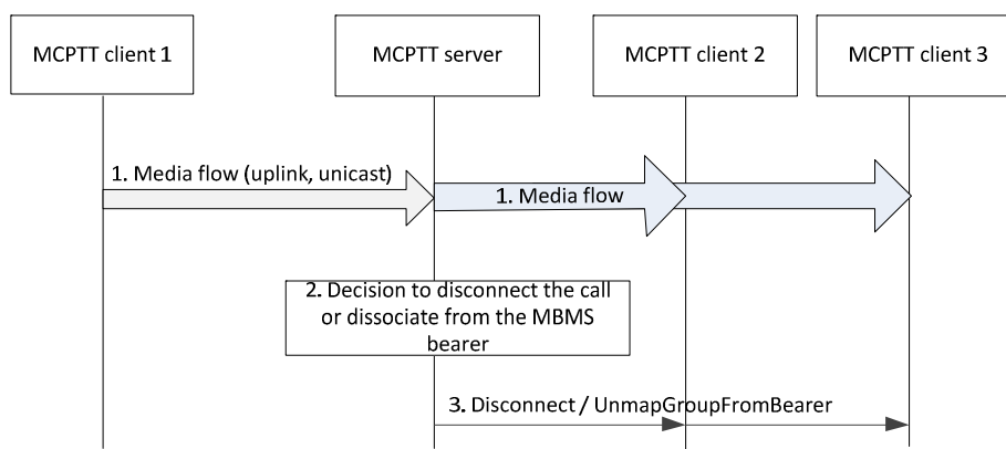
Figure 10.10.4.2-2: Chat group call disconnect on MBMS bearer
