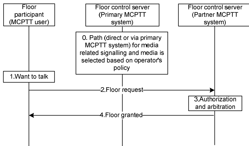
Figure 10.12-1: Media related signalling communication
