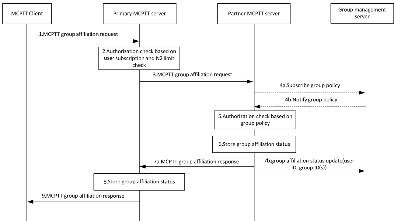
Figure 10.3.3.2.2-1: Affiliation for an MCPTT group defined in partner MCPTT system
