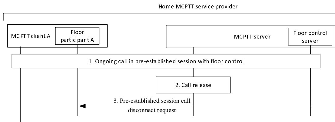
Figure 10.5.3.5.1-2: Disconnect procedure
