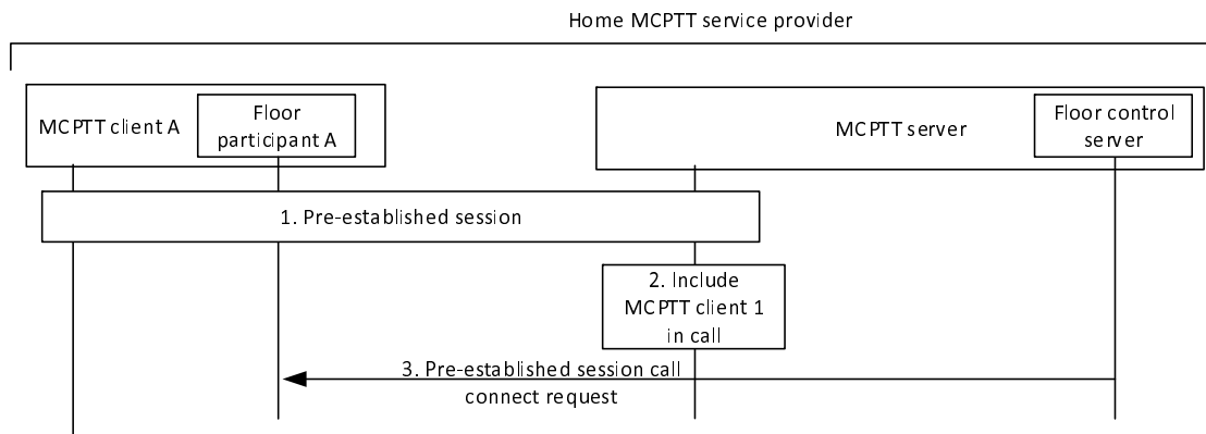
Figure 10.5.3.5.1-1: Connect procedure
