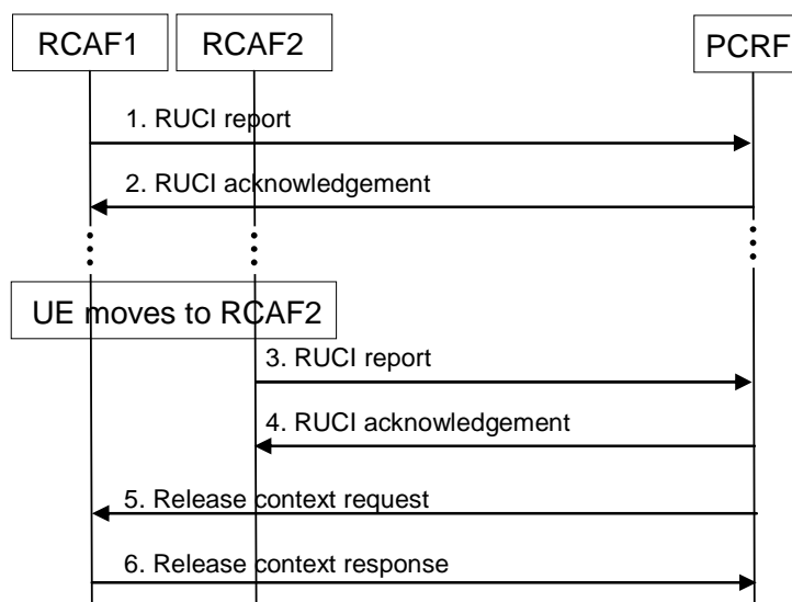
Figure 7.10.3: UE mobility from RCAF1 to RCAF2 in case UE is affected by congestion at RCAF2 after the UE was earlier affected by congestion at RCAF1
