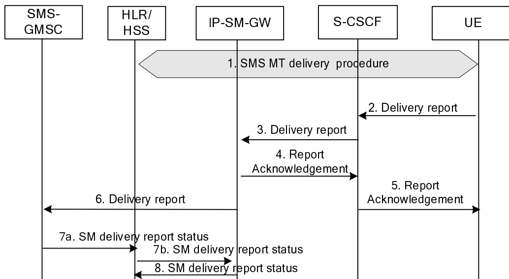
Figure 6.5: Delivery report procedure
