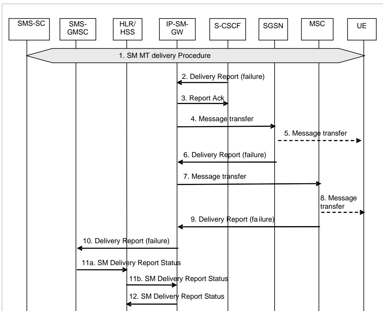
Figure 6.5a: Unsuccessful SMS MT delivery procedure
