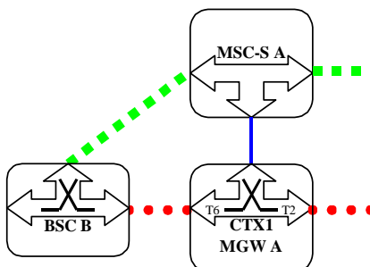
Figure 8.23 Subsequent Inter-MSC GSM to GSM Handover back to the Anchor MSC (network model)
