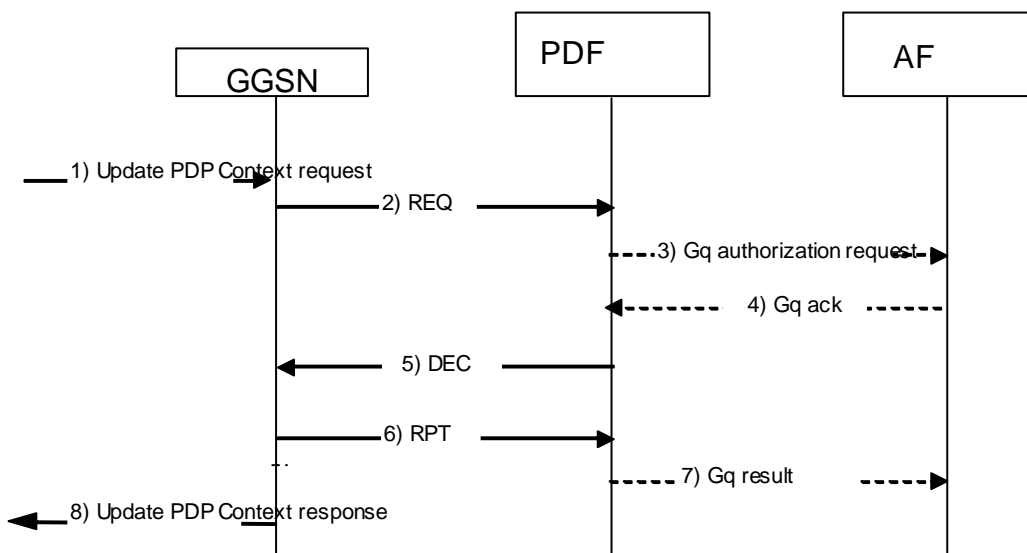
Figure 14a: Authorization of PDP Context Modification
