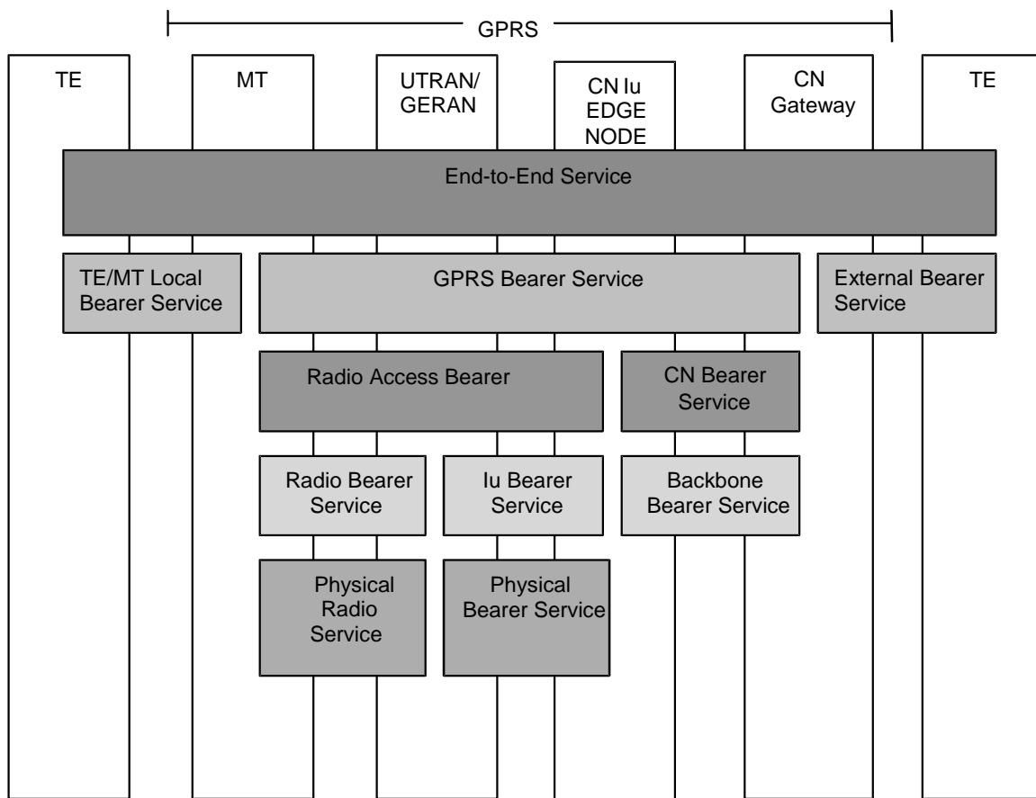
Figure 1: End-to-End QoS Architecture
