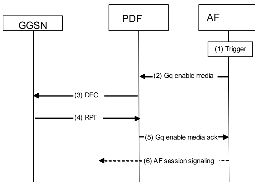
Figure 11: Enable media procedure
