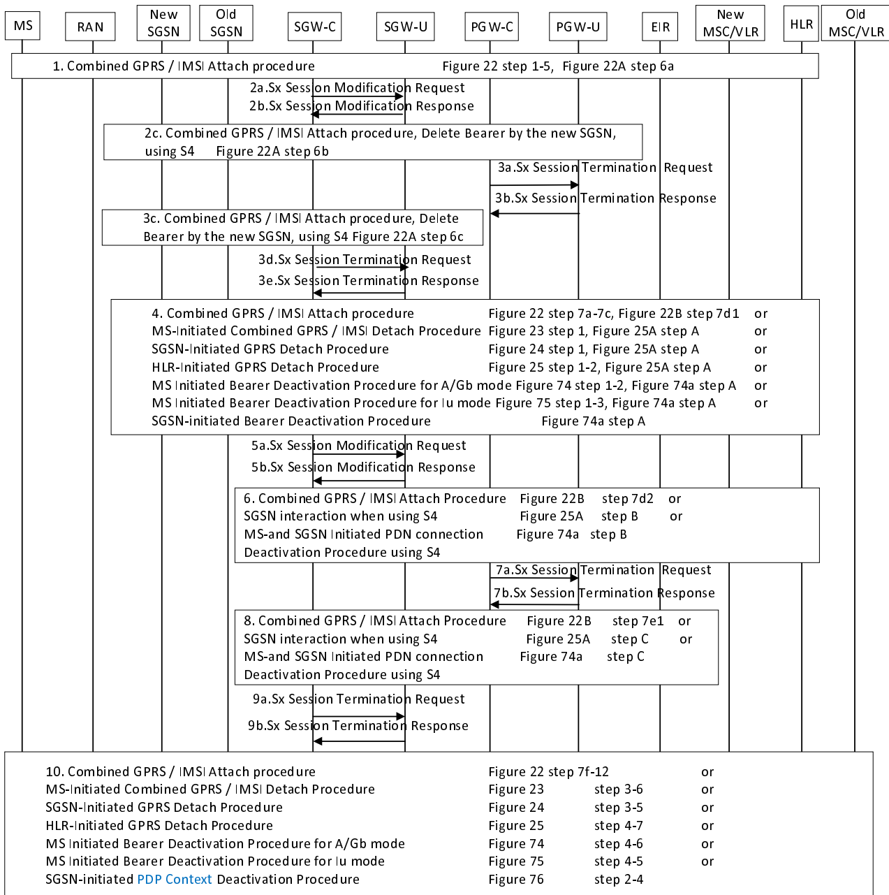
Figure 6.3.4.1-1: Interaction between CP and UP function with PDN connection deactivation Group 1
