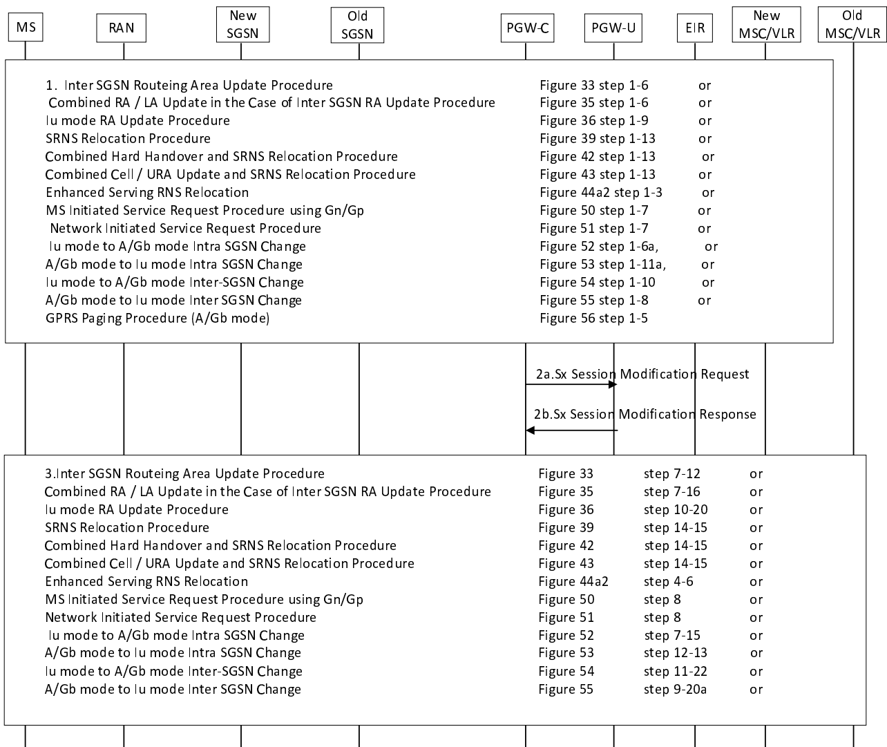
Figure 6.3.4.2.2-1: Interaction between CP and UP function with PDN connection modification, Group
