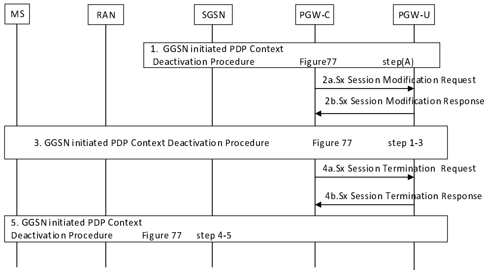
Figure 6.3.4.1.2-2: Interaction between CP and UP function with PDN connection deactivation Group 2
