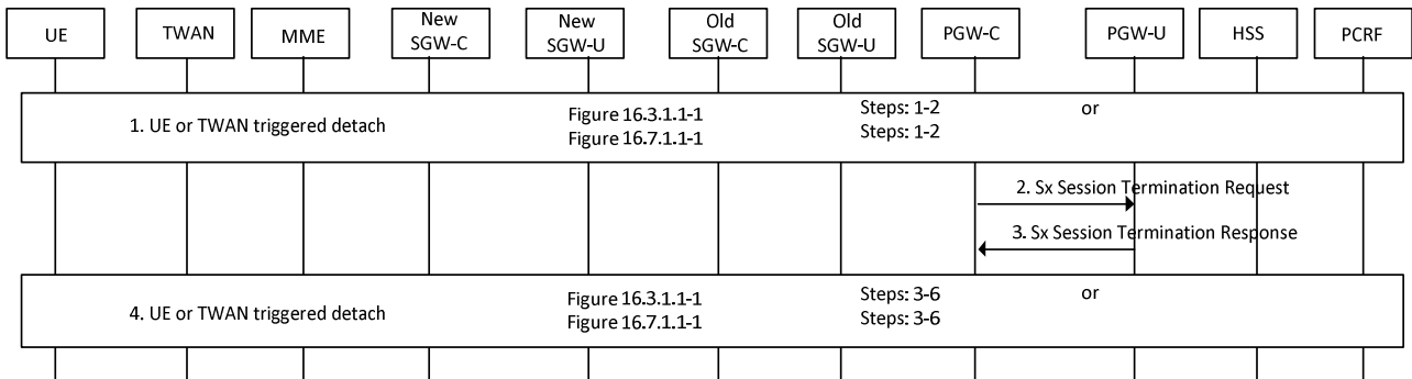
Figure 6.3.3.4-1: Interaction between CP and UP function with release of GTP based S2a
