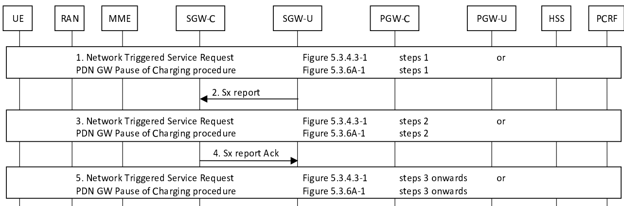
Figure 6.3.1.5-1: Interaction between CP and UP when downlink data is buffered in the UP function
