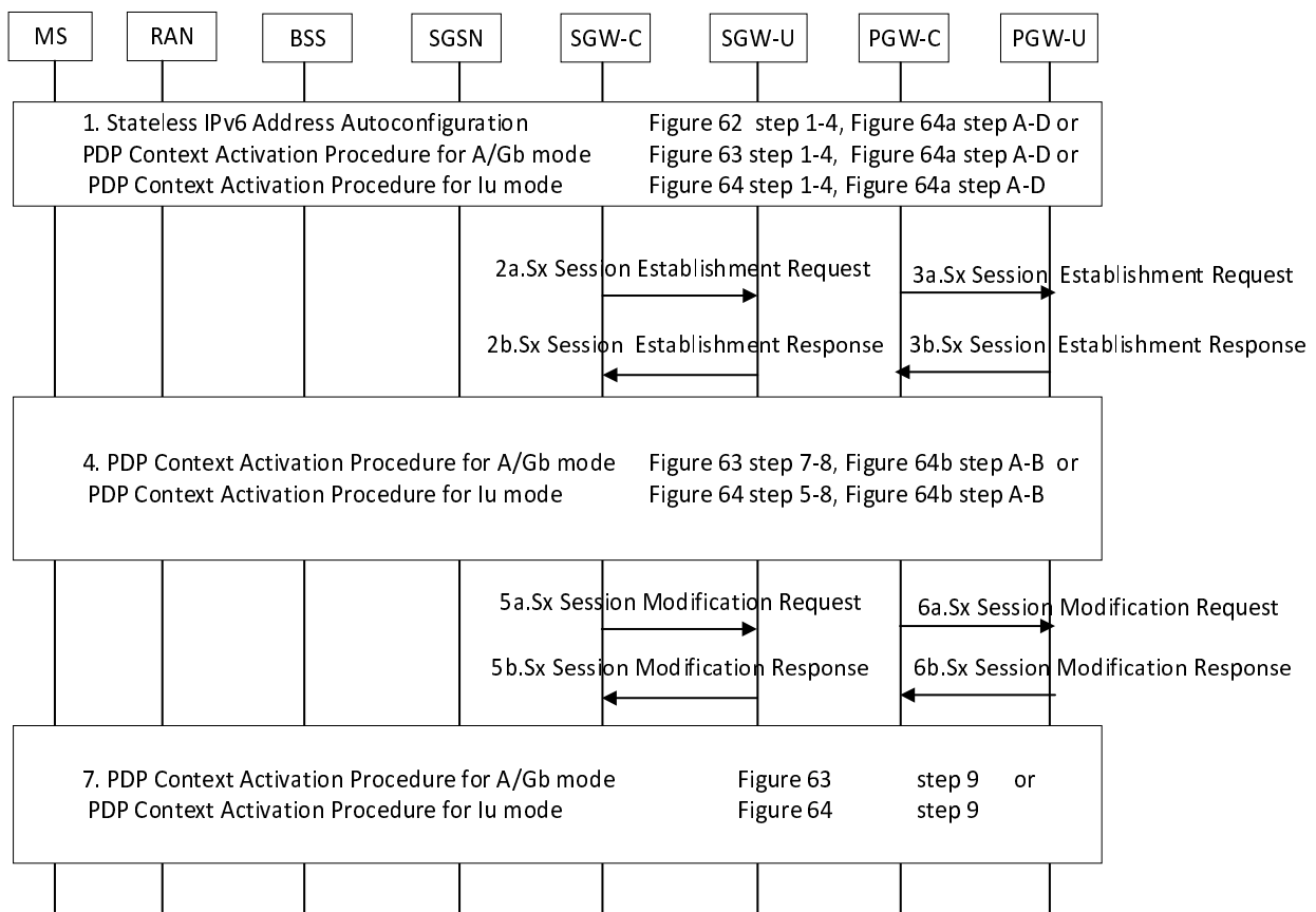
Figure 6.3.4.3-1: Interaction between CP and UP function with PDN connection establishment
