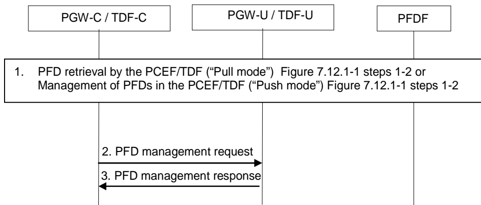
Figure 6.3.2.4-1: Interaction between CP and UP function with PFD management
