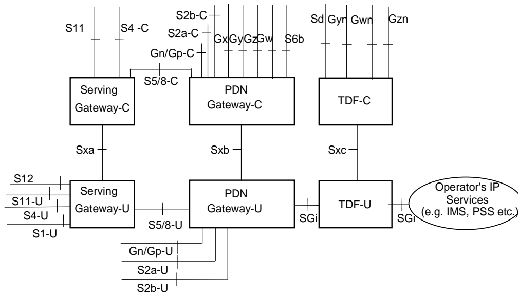
Figure 4.2.1-1: Architecture reference model with separation of user plane and control plane for non-roaming and roaming scenarios
