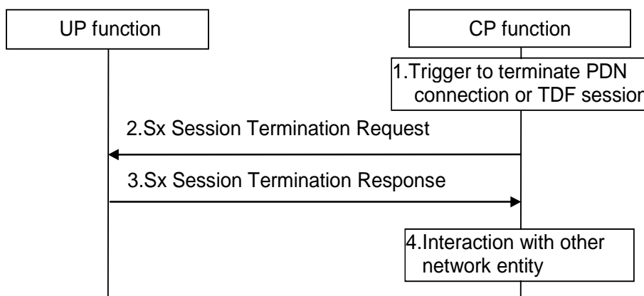
Figure 6.2.4-1 Sx session termination procedure
