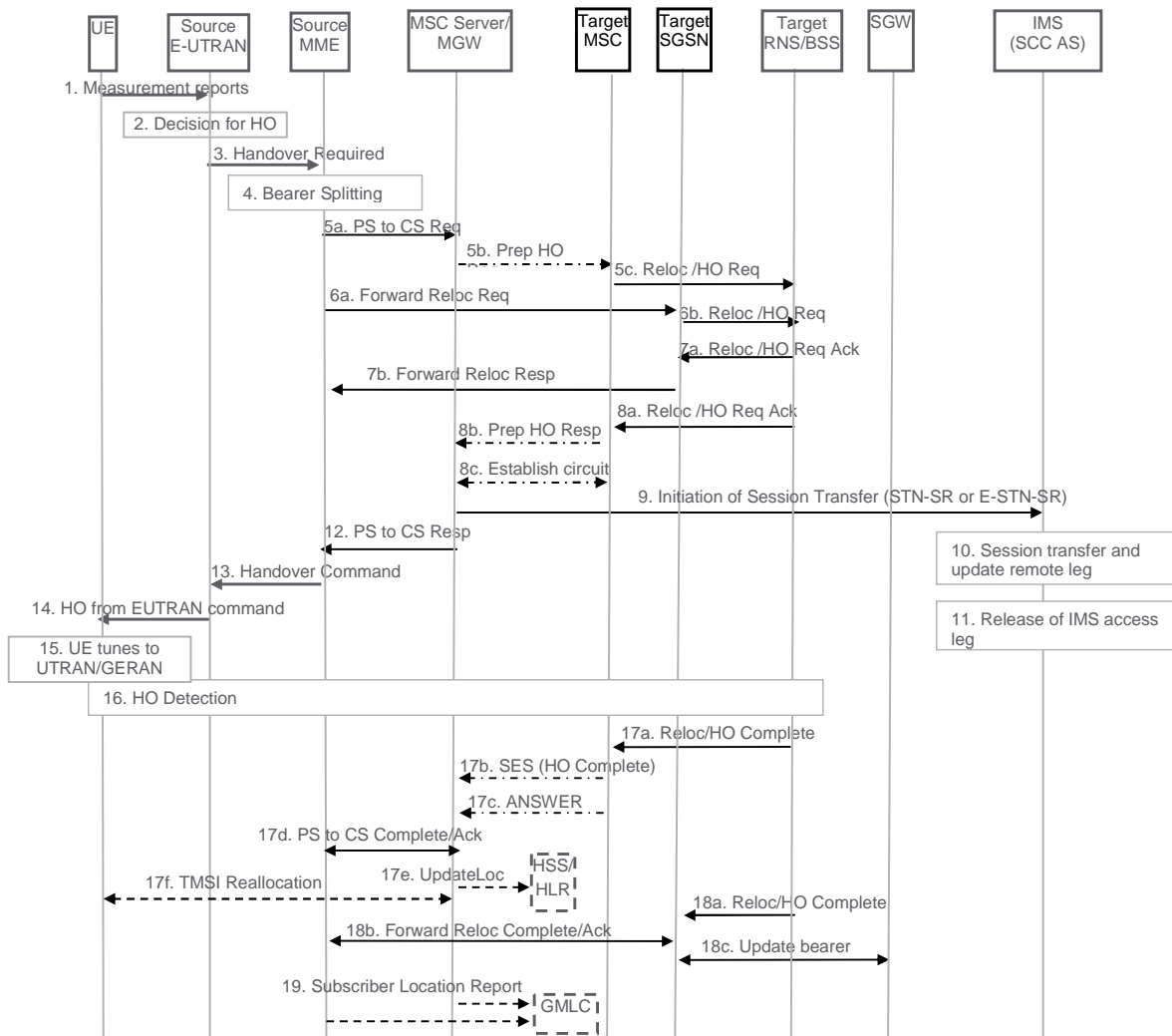
Figure 6.2.2.2-1: SRVCC from E-UTRAN to UTRAN with PS HO or GERAN with DTM HO support
