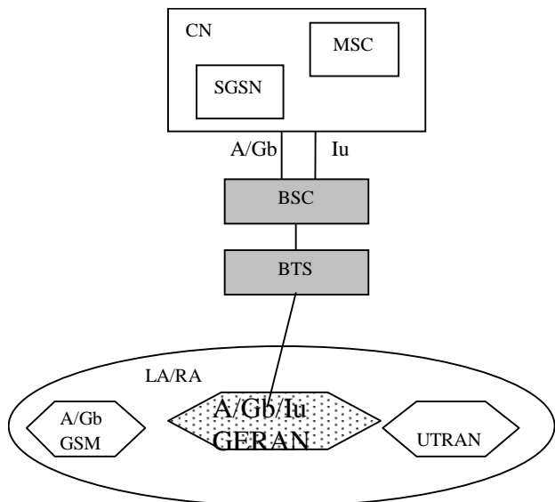
Figure 6.2a: Combined Iu/A/Gb Cell with Combined CN nodes
