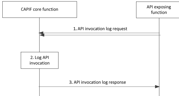
Figure 8.19.3-1: Procedure for logging service API invocations
