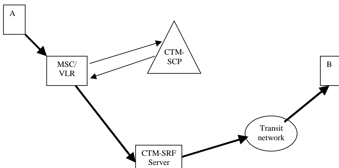
Figure C.4: Mobile originating call routing overview
