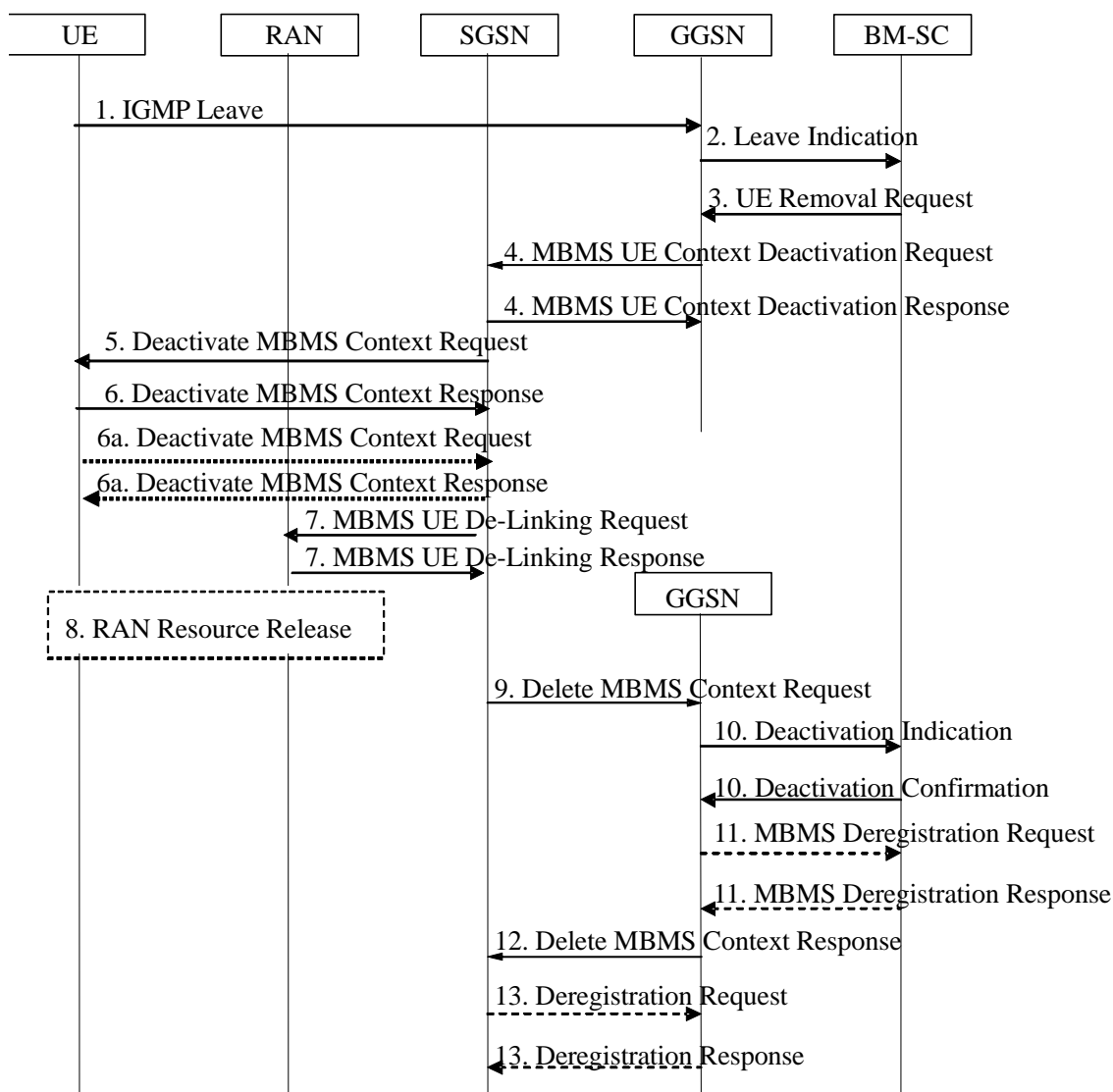
Figure 13: MBMS Multicast Service Deactivation
