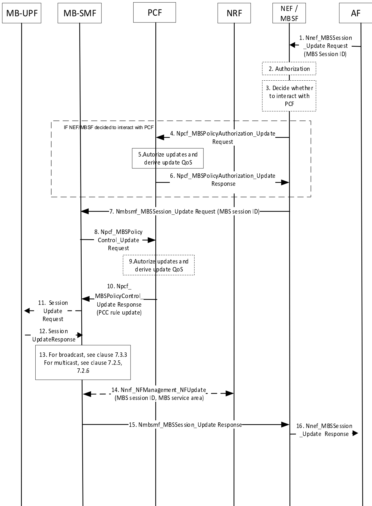
Figure 7.1.1.7-1: MBS Session Update with PCC
