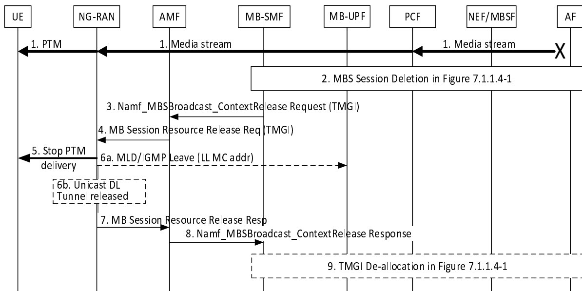
Figure 7.3.2-1: MBS Session Release for Broadcast
