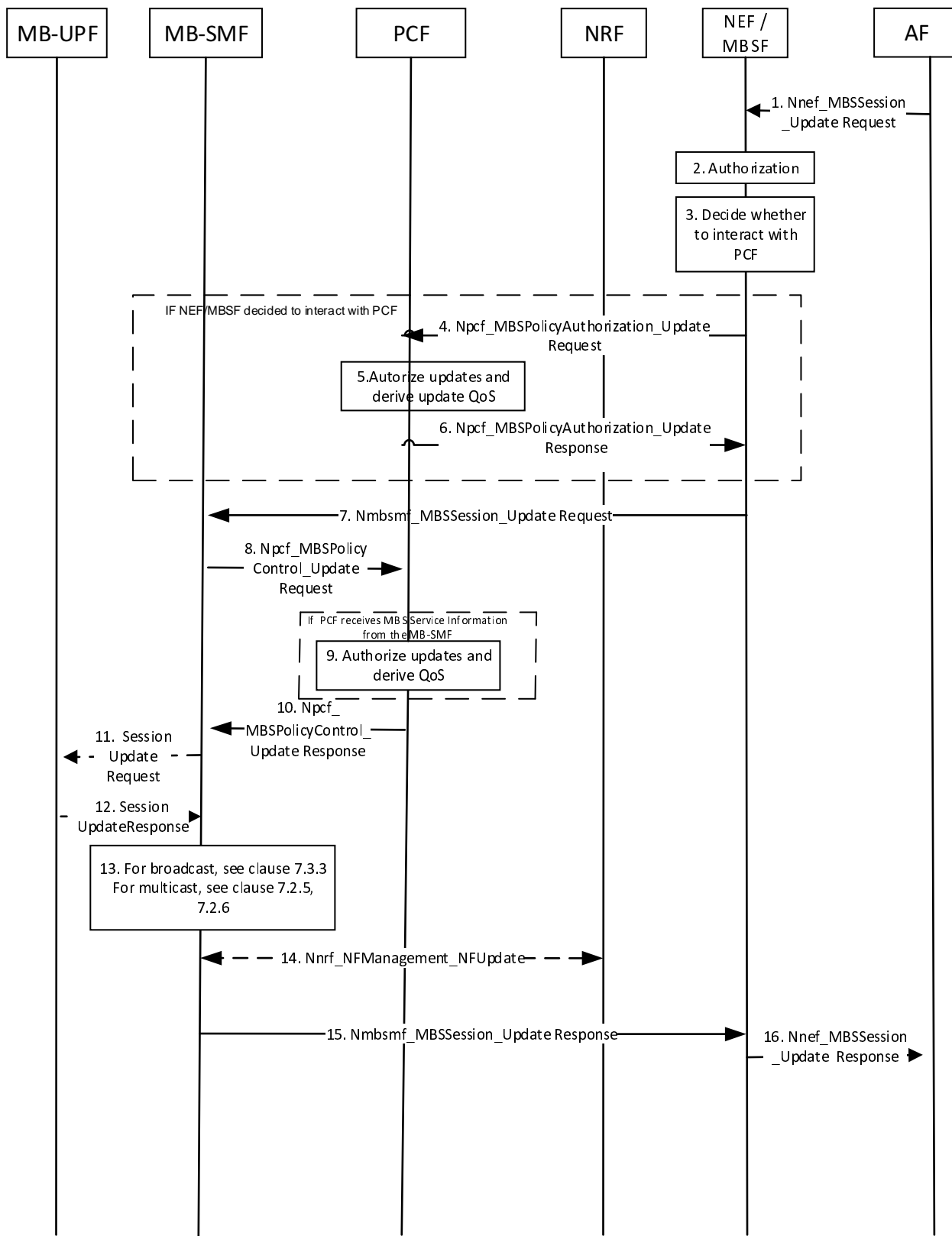
Figure 7.1.1.7-1: MBS Session Update with PCC
