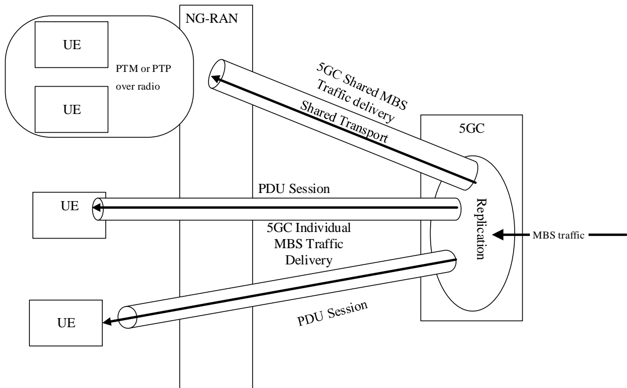
Figure 4.1-1: Delivery methods
