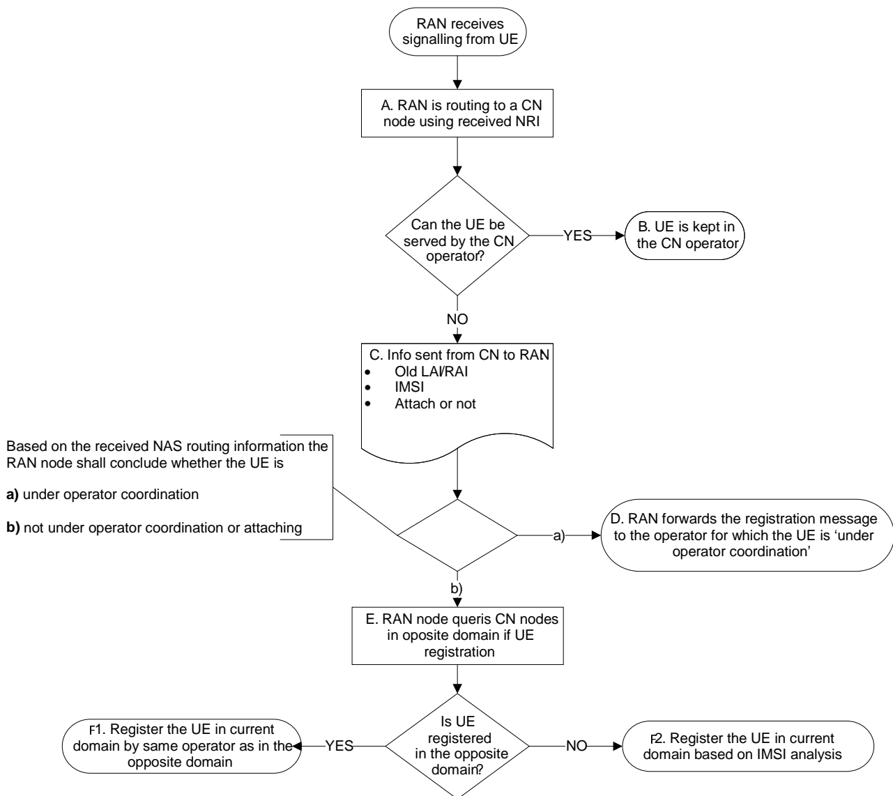
Figure A.4-1: Flow diagram for CSPA Coordination
