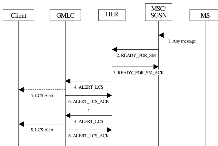
Figure 9.y: LCS Client Alerting procedure
