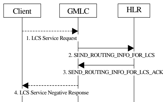
Figure 9.x: MT-LR routing procedure
