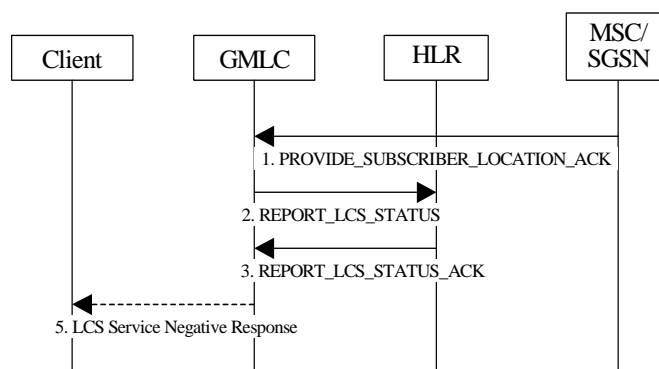
Figure 9.z: UE Presence Notification procedure
