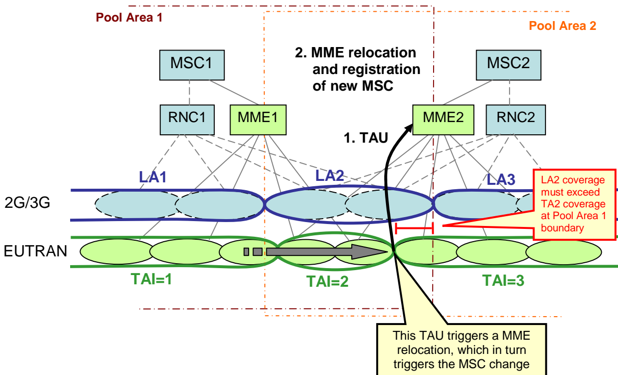
Figure A.1-1: Solution 1: Overlapping Pool Areas with 2G/3G coverage > EUTRAN coverage at Pool Area Boundaries
