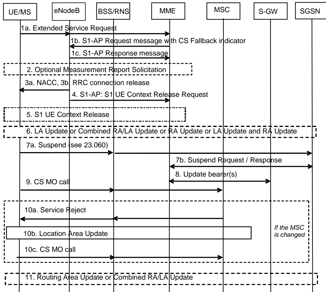
Figure 6.3-1: CS Call Request in E-UTRAN, Call in GERAN/UTRAN without PS HO
