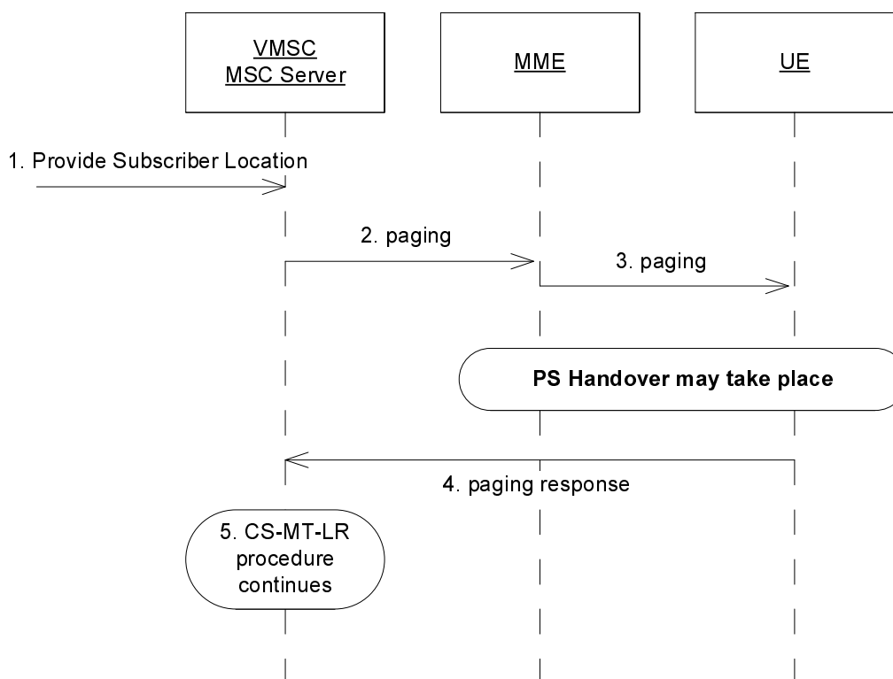
Figure 8.3.2.1-1: MT-LR procedure if UE is not in IMS VoIP session
