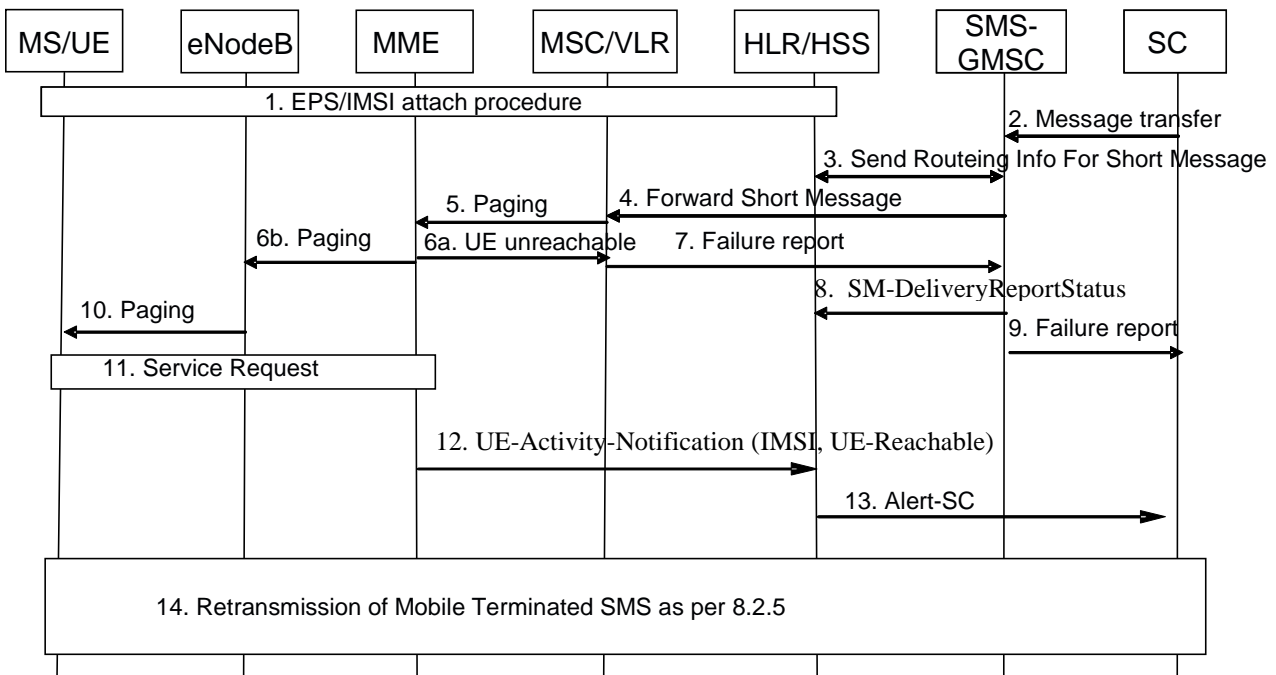
Figure 8.2.4a-1: Mobile terminating SMS in extended idle mode DRX
