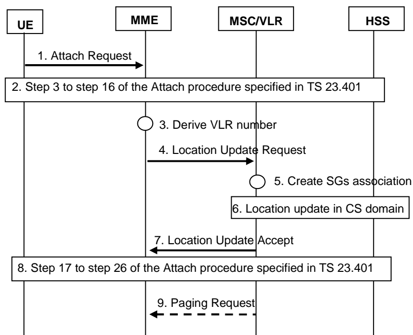
Figure 5.2-1: Attach Procedure
