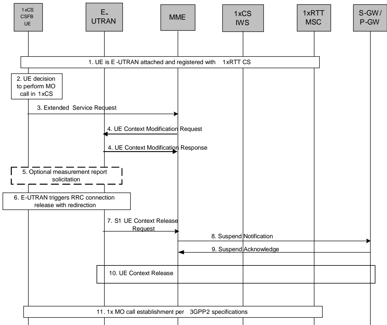
Figure B.2.2-1: CS MO call using fallback to CDMA 1x RTT network
