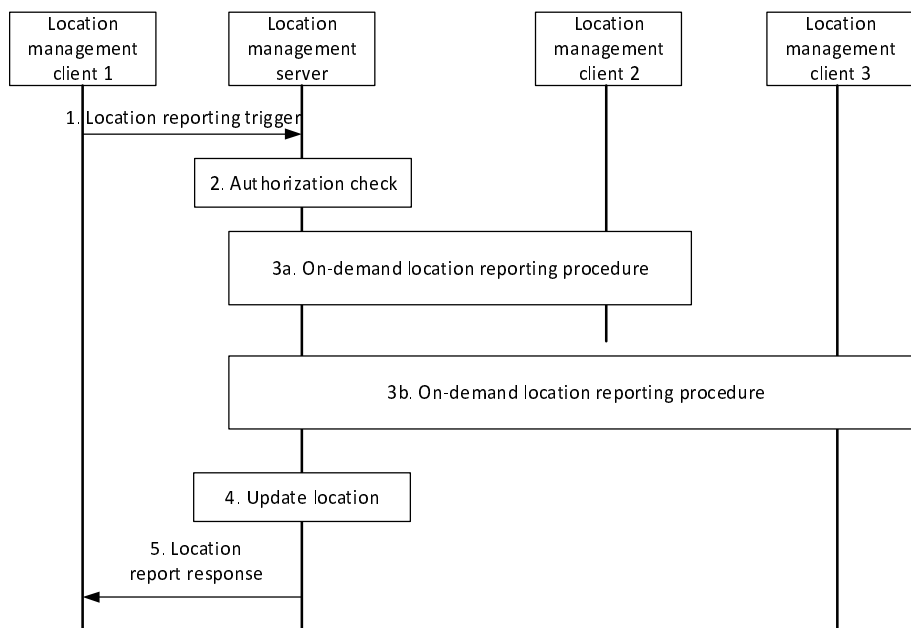
Figure 10.9.3.8.1-1: One-time location information report for shared functional aliases
