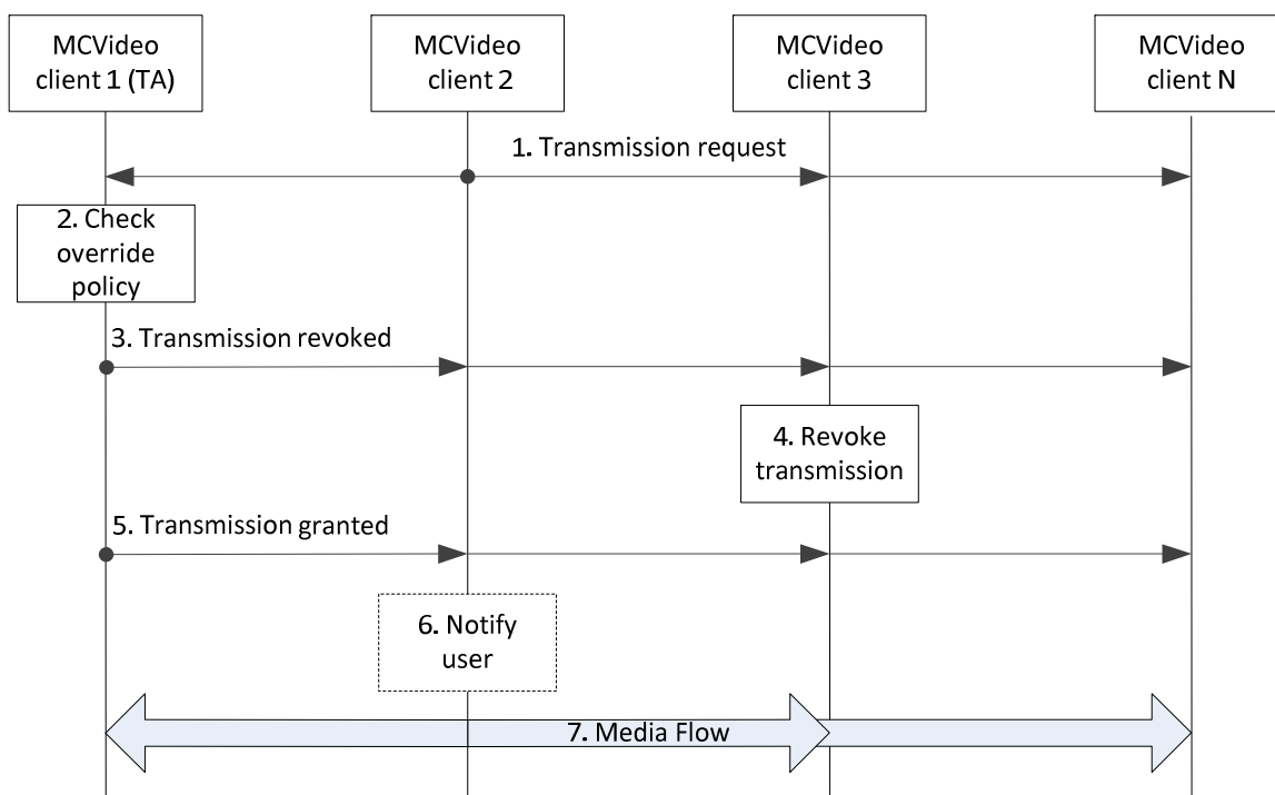
Figure 7.7.2.7-1: Transmission override
