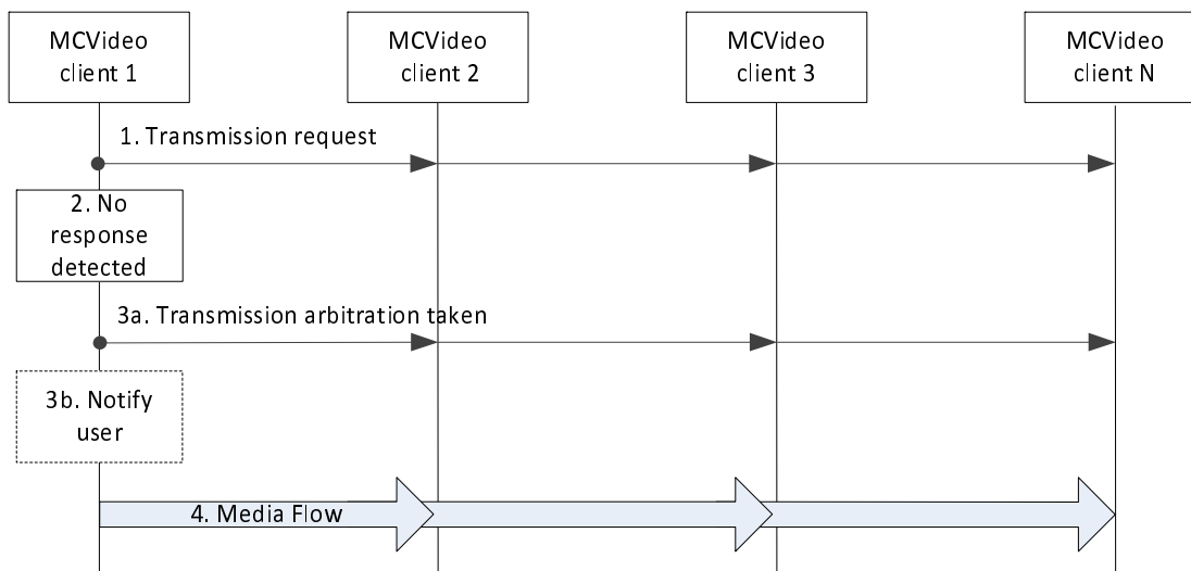
Figure 7.7.2.3-1: Initializing transmission control, single arbitrator case
