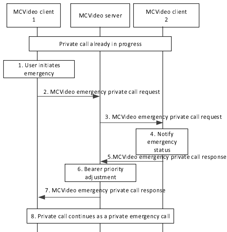
Figure 7.2.2.4.2-1: MCVidéo private call upgrade
