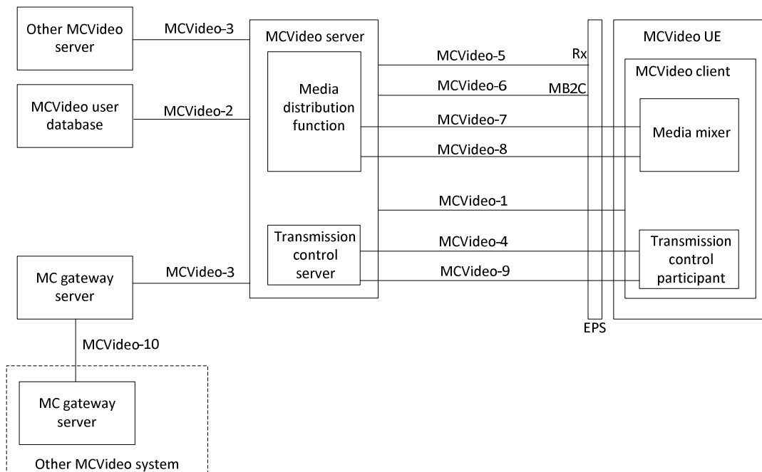
Figure 6.1.1-1: Functional model for application plane of MCVideo service
