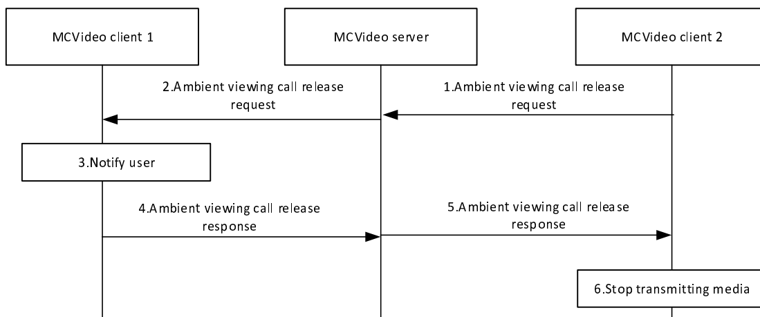
Figure 7.6.3.5-1: Ambient viewing call release – "viewed to" user initiated
