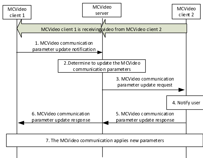
Figure 7.17.3.4-1: Receiving user triggered MCVidéo adaptation in private communication
